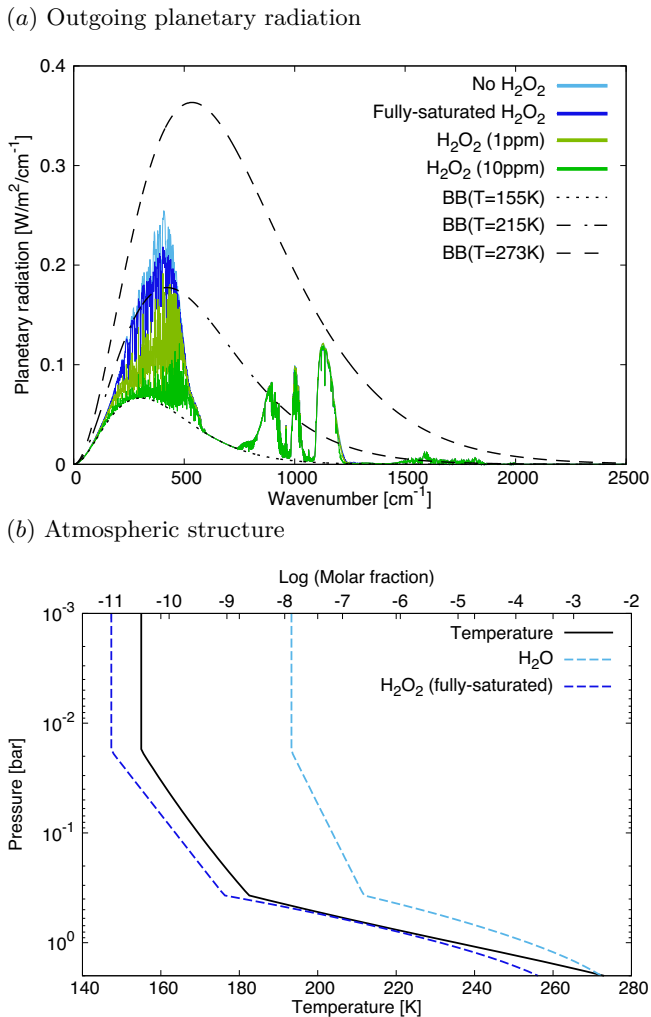
Figure 5. Impact of H 2 O 2 on the outgoing planetary radiation for a surface pressure of 2 bar and a surface temperature of 273 K. Panel (a) — the outgoing planetary radiation as a function of wavenumber for the atmospheres without H 2 O 2 and with different amounts of H 2 O 2 . The black dashed curves show the blackbody radiation, the temperatures of which are indicated, BB( T ). Panel (b) — the temperature-pressure profile and the vertical distributions of H 2 O and saturated H 2 O 2 in the atmosphere.
