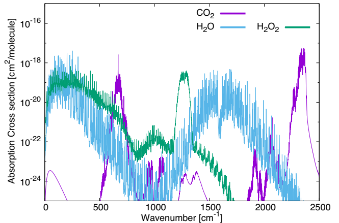
Figure 1. Absorption cross sections of three oxidized gases, \text{CO}_2 (magenta), \text{H}_2\text{O} (cyan), and \text{H}_2\text{O}_2 (green) at 250 K and 1 bar, as functions of wavenumber. These cross sections are produced using the line profile calculation code EXOCROSS (Yurchenko et al. 2018). The absorption data and the assumed line profiles are described in Sec. 2.
