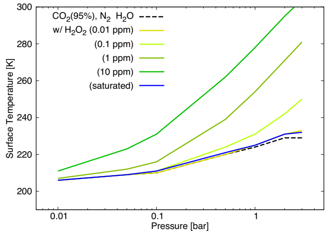
Figure 6. Surface temperature as a function of surface pressure. The dashed curve represents the atmosphere without H 2 O 2 while the solid curves show the atmospheres containing a saturated amount and vertically constant molar fractions of H 2 O 2 . Note that, the case of 0.01 ppm of H 2 O 2 (yellow) is almost identical to those of saturated- (blue) and free-H 2 O 2 (black).
