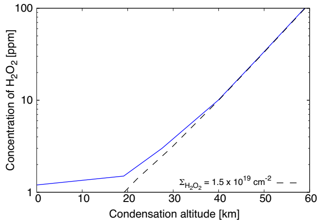
Figure 7. The concentration of H 2 O 2 necessary to warm the planetary surface to 273 K in the 2-bar atmosphere as a function of the condensation altitude (see the text for the definitions of each term). The dashed line represents the column density of H 2 O 2 with a constant concentration to reach \Sigma_{\text{H}_2\text{O}_2} = 1.5 \times 10^{19} \text{ cm}^{-2} .
