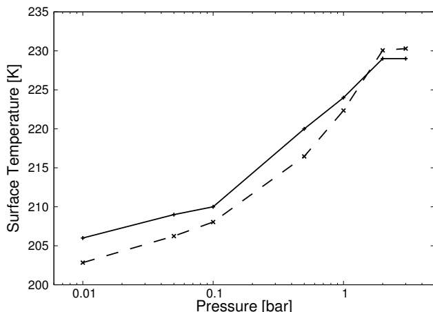
Figure 4. Surface temperature as a function of surface pressure for wet \text{CO}_2(95\%)\text{-N}_2(5\%) atmospheres, comparing the result calculated by our model (solid) against the result of Ramirez et al. (2014) (dotted).
