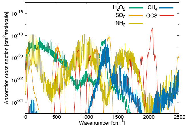
Figure 2. Absorption cross sections of \text{H}_2\text{O}_2 (green) and four greenhouse gases, \text{SO}_2 (orange), \text{NH}_3 (yellow), \text{CH}_4 (blue) and \text{OCS} (red) at 250 K and 1 bar, as functions of wavenumber. These cross sections are calculated using EXOCROSS (Yurchenko et al. 2018) and HITRAN2012 (Rothman et al. 2013), assuming a Voigt profile truncated at 25\text{ cm}^{-1} from the line center.
