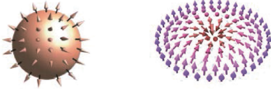
Figure 2. On left: a spin configuration with n_1^2 + n_2^2 + n_3^2 = 1 dispatched on a 2-sphere. On right: a two space dimensional magnetic skyrmion given by the stereographic projection of \mathbb{S}^2 to plane.
