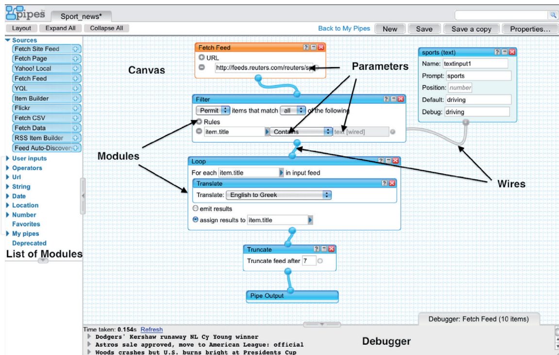
Figure 1. Yahoo! Pipes.
