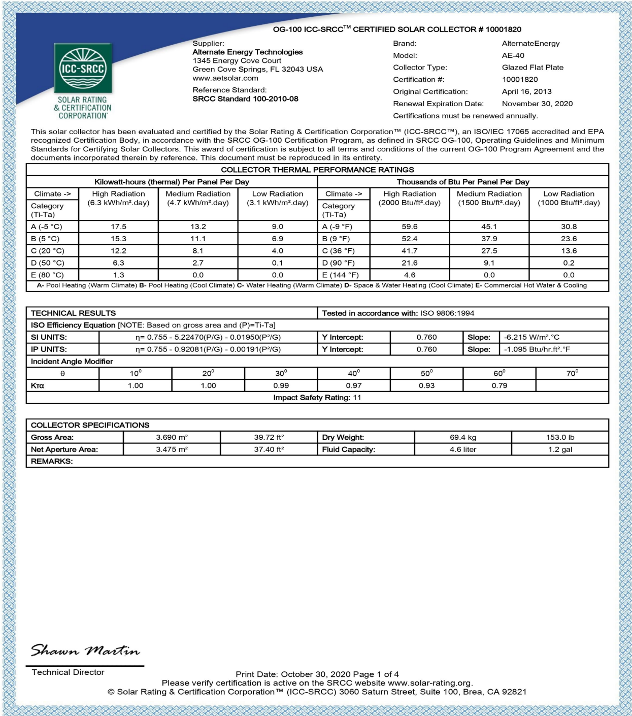
Figure 10: OG-100 Certification for Model AE-40 by Alternate Energy Technology[4]
