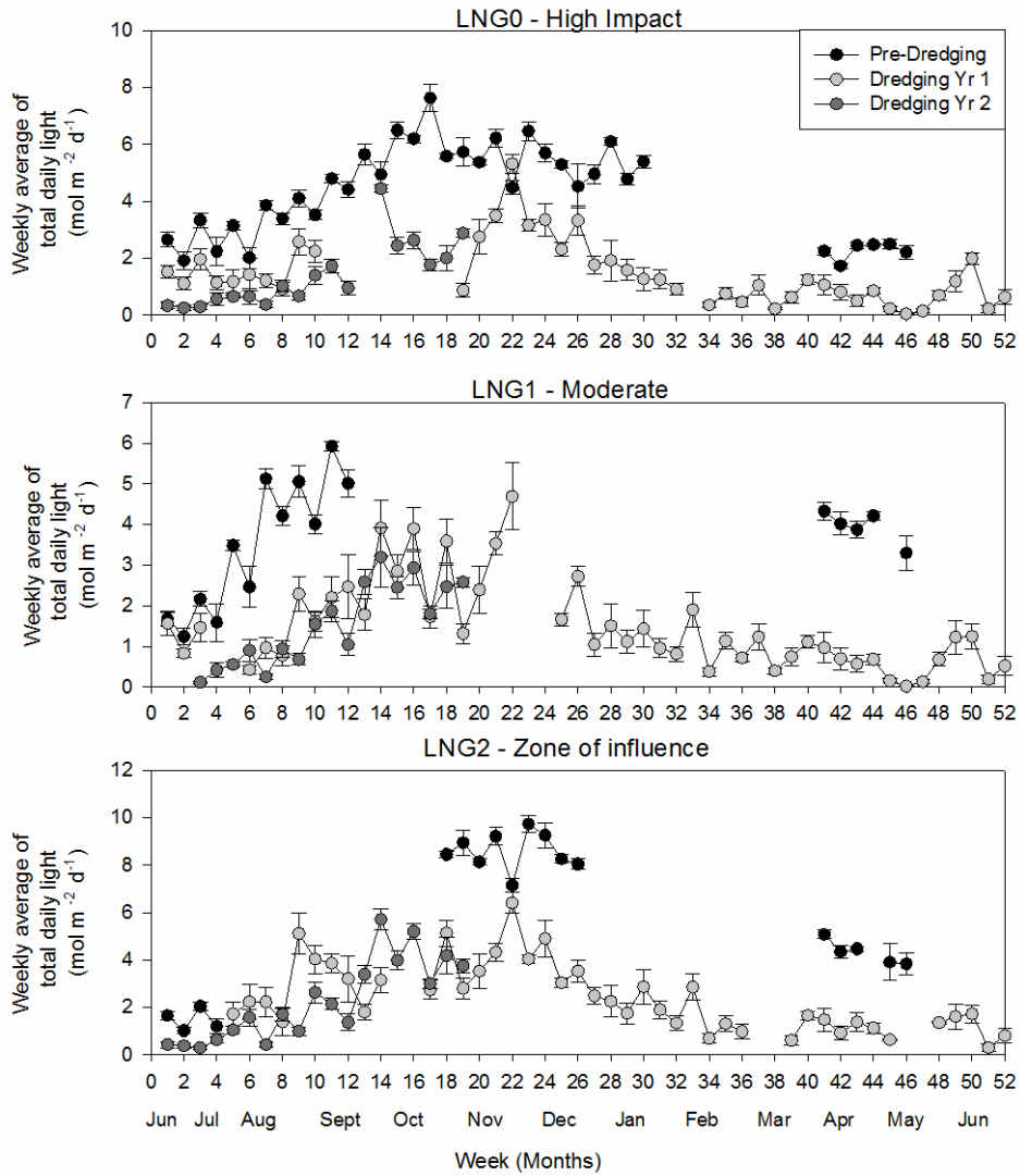
Figure 5: Daily total light ( \text{mol m}^{-2} \text{d}^{-1} ) for sites closest to the dredge, averaged over 7 days from 20 June 2009 (week 1) to 18 May 2010 (Week 52) for pre-dredging data, 19 May 2010 to 18 May 2011 for Year 1 dredging data, and then 19 May 2011 to 24 October 2011 for Year 2 dredging data. Only weeks with 6 or more daily readings were included.
