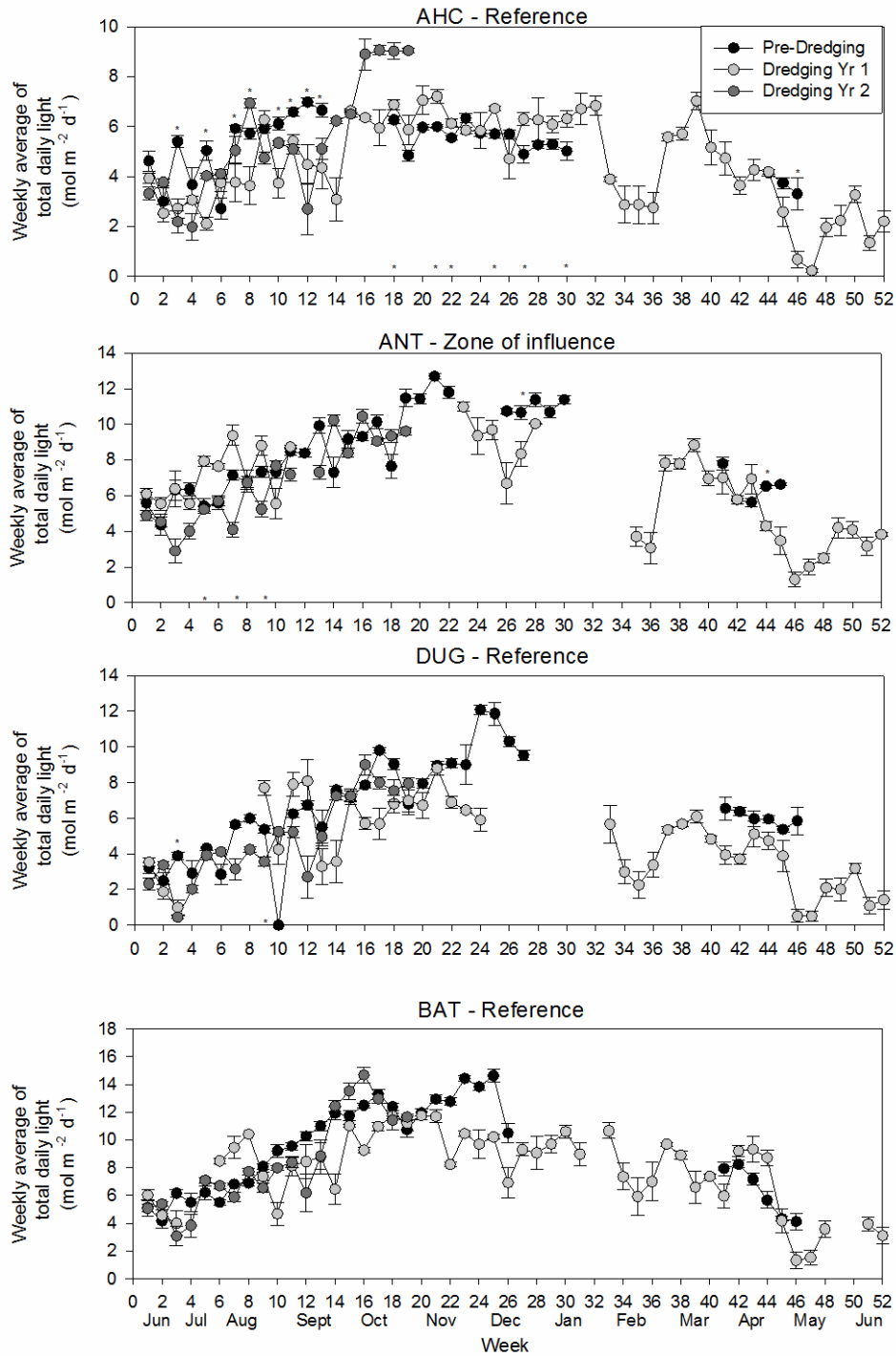
Figure 6: Daily total light ( \text{mol m}^{-2} \text{d}^{-1} ) for sites furthest from dredge, averaged over 7 days from 20 June 2009 (week 1) to 18 May 2010 (Week 52) for pre-dredging data, 19 May 2010 to 18 May 2011 for Year 1 dredging data, and then 19 May 2011 to 24 October 2011 for Year 2 dredging data. Only weeks with 6 or more daily readings were included.
