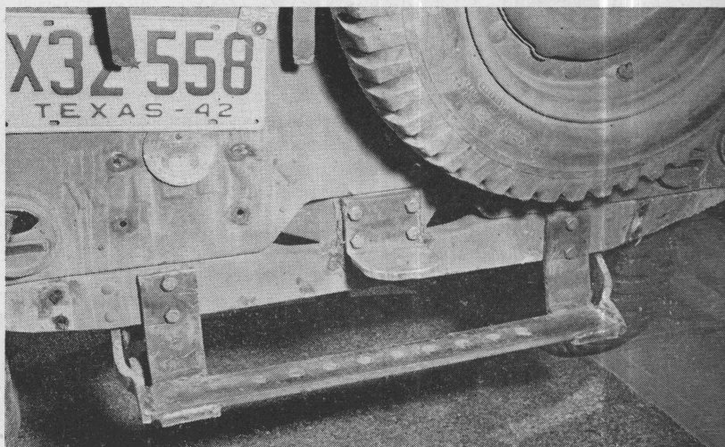
Fig. 2. Drawbar and trailer hitches mounted on military jeep. Either a ball or pin can be used with the trailer hitch.
