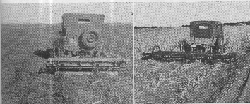
Fig. 3. Left—Military jeep pulling a two-row tractor type stalk cutter cutting cotton stalks. The cutter is hitched to the left end of the drawbar and the left wheels of the jeep are almost running on the row of stalks. Right—The Universal jeep pulling a four-row homemade stalk cutter cutting sorghum stubble. The cutter is hitched to the center of the drawbar of the jeep, thus making it necessary to drive with the wheels running directly on the two center rows.
