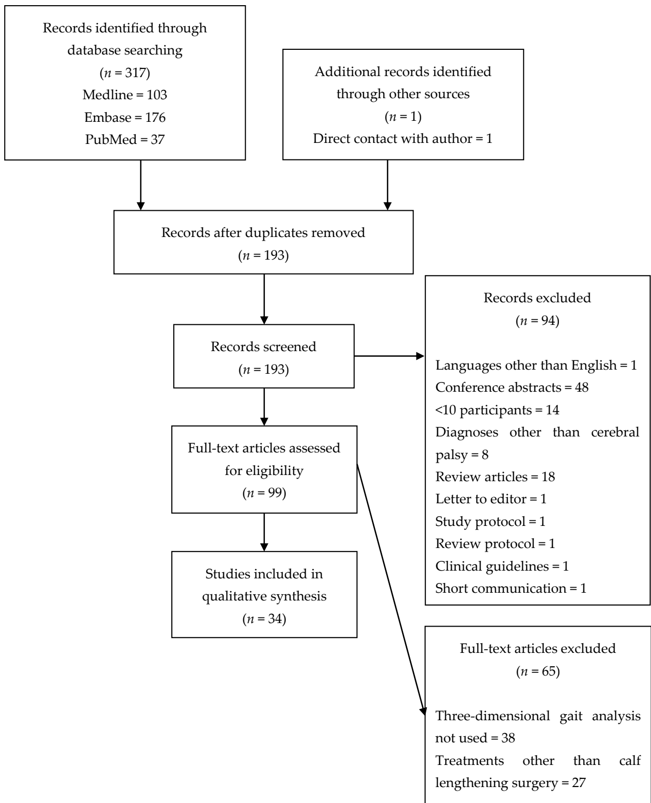
Figure 3. PRISMA diagram.
