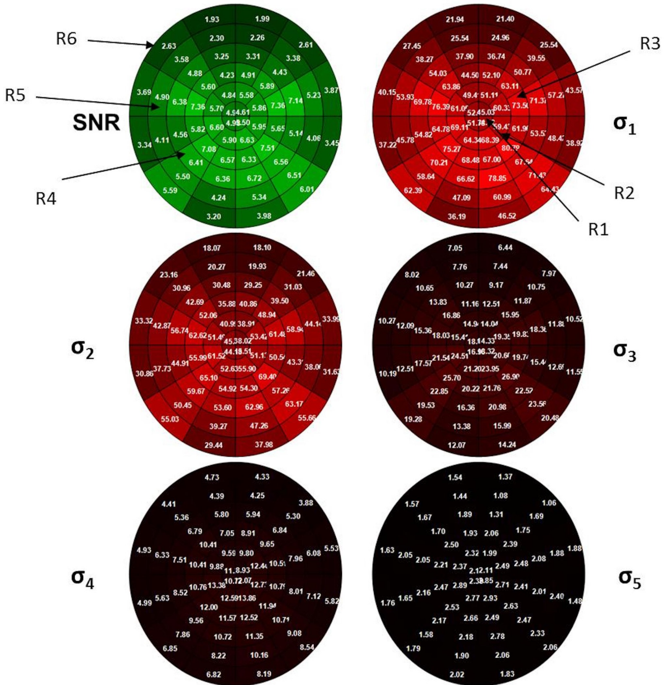
Fig 2. Signal-to-noise ratio (SNR) values (green) and singular values ( \sigma_1, \dots, \sigma_5 ) for the averaged control group for each sector of the visual field. When the values tend to zero, the colour of the sector is darker. R1, . . . R6: concentric rings.
