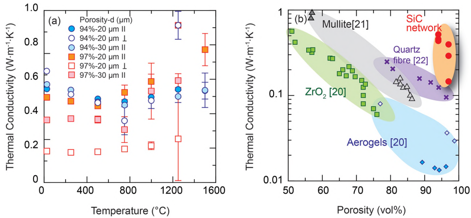
Figure 2. a) The thermal conductivities in the direction parallel (||) and perpendicular (⊥) to the layers remain low with temperature up to 1500 °C although it tends to increase at higher temperatures for the materials with larger pores. b) The thermal conductivity (room temperature values) of the SiC networks is comparable to other porous thermally insulating ceramics. Aerogels have lower thermal conductivity and are lighter but they are also weaker (data from refs. [20–22]).
