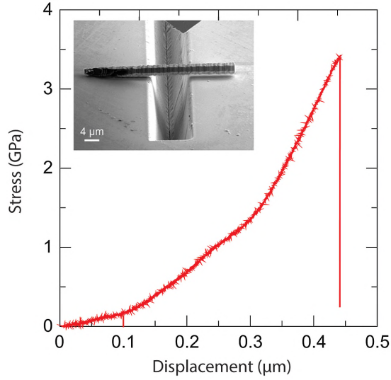
Figure 5. Stress/strain curve from a single fiber bending test performed in situ in the scanning electron microscope (inset is a scanning electron microscopy showing the set-up). The initial nonlinearity of the curve is likely due to fiber movement under the indenter.
