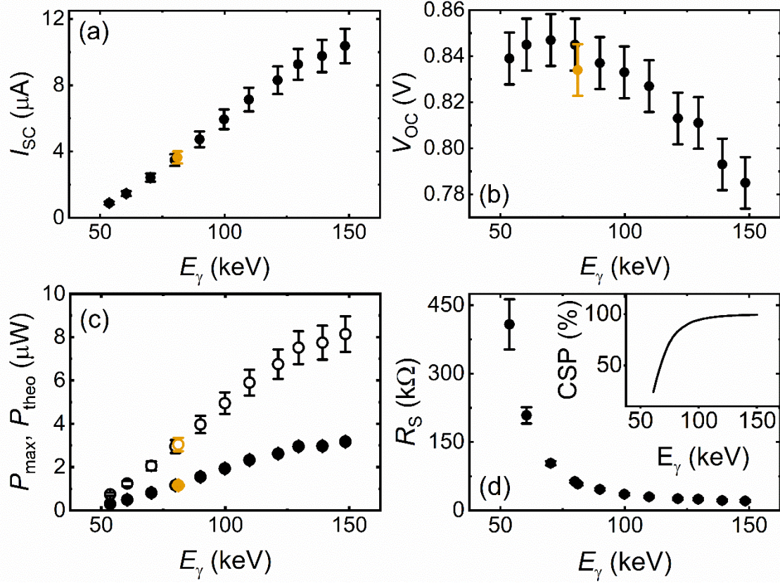
Figure 5: Parameters extracted from Figure 4 . (a) is the DGV short-circuit current I_{sc} . (b) is the open-circuit voltage V_{oc} . The V_{oc} is not legitimately treated by this scaling method, hence the gradual decrease with energy; this is due to the decreasing flux with energy in the raw data. (c) shows the maximum power P_{max} ( closed circles ) and theoretical maximum power P_{theo} = I_{sc} \times V_{oc} ( open circles ). (d) shows series resistance R_s of the device. Also shown, for comparison, are calculated cross-section data for the proportion of interactions that are Compton scattering events [49] ( inset ). The measurement taken after the others, at 81.1 eV, is shown in orange for clarity in subfigures (a-c) , but not in (d) as time information is lost in the resistance extraction process.
