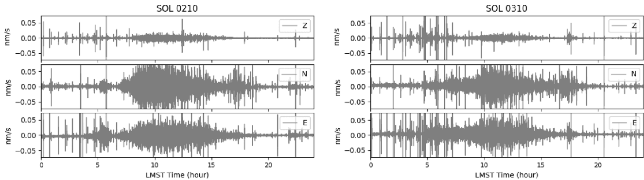
Figure 2. Continuous signals in velocity recorded by the three components of InSight's broadband seismometer on Mars (top: Z, middle: N, bottom: E). On sol 210 (left) and 310 (right) filtered between 0.03 and 1 Hz.
