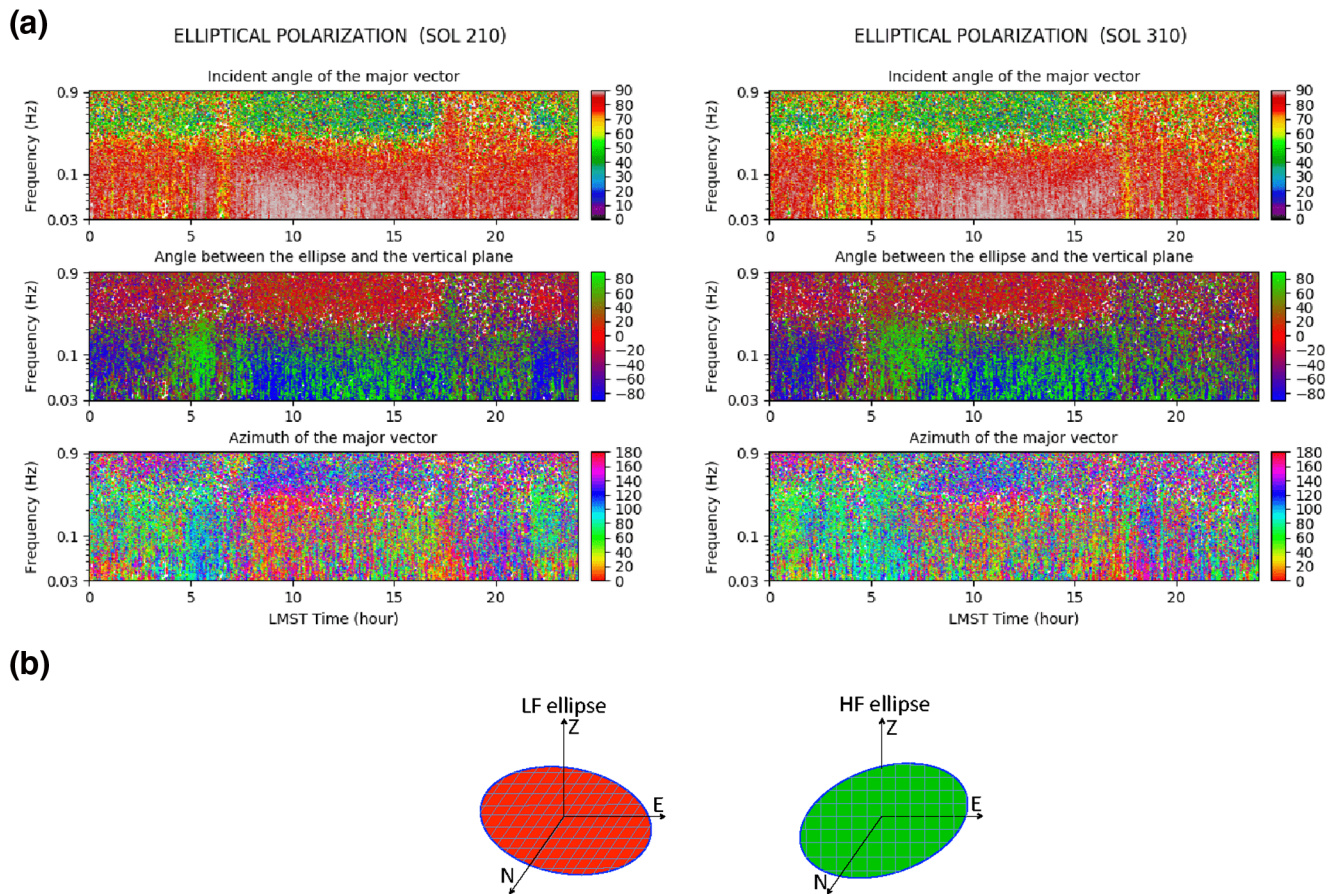
Figure 7. (a) For signals with elliptical polarization, incident angle of the major axis (top), angle between the ellipse and the vertical plane (middle), and azimuth of the major vector (bottom) as a function of LMST time and frequency for sol 210 (left) and 310 (right). Angles are all in degrees. Azimuth are between 0^\circ and 180^\circ with an ambiguity of 180^\circ . A sketch of the high frequency horizontal and low frequency vertical ellipses of polarization is shown in (b).
