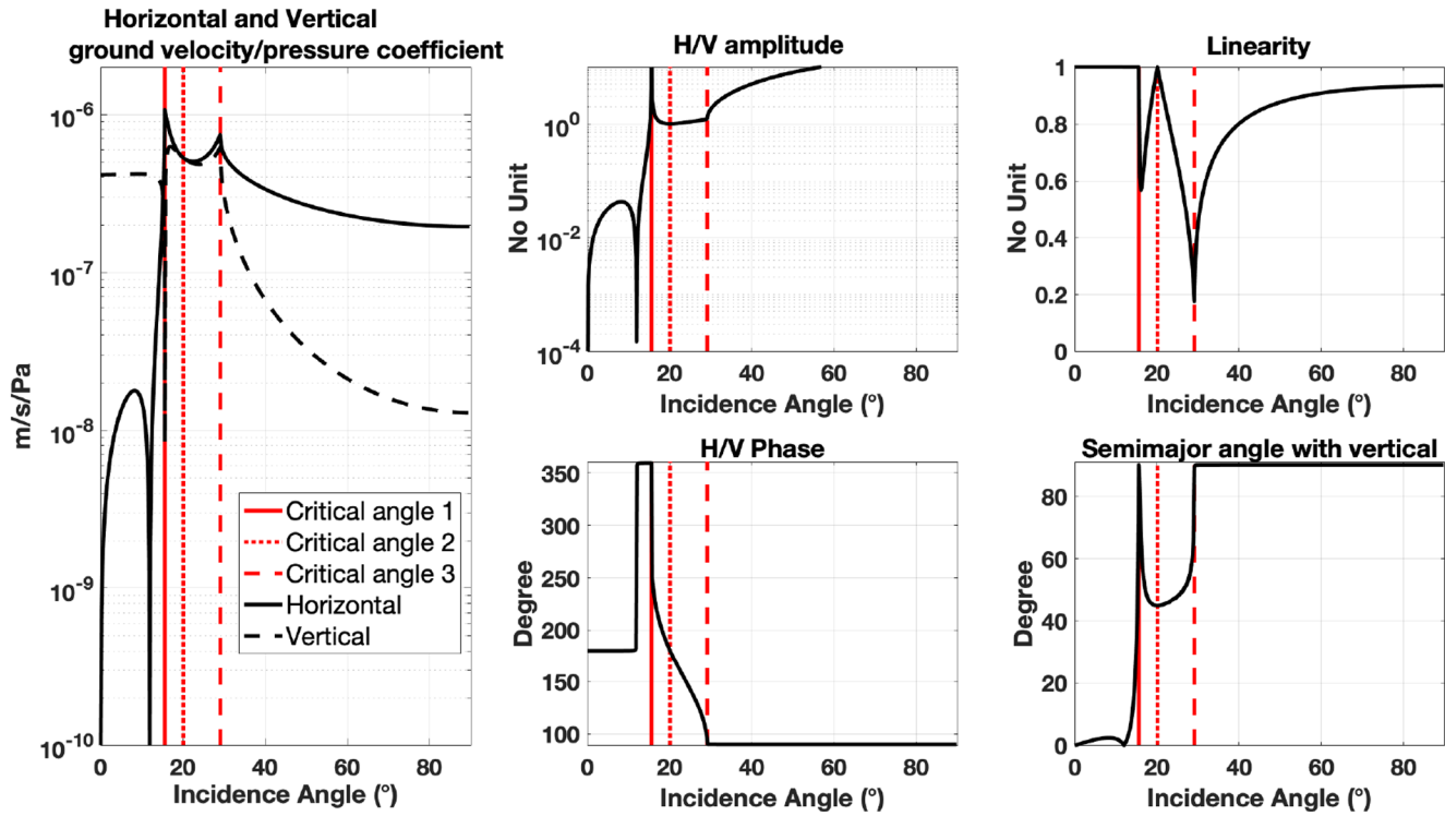
Figure 18. Transmission coefficient between the pressure amplitude of an acoustic wave and the horizontal and vertical ground velocity and impacts in terms of ground ellipticity. The left figure provides the transmission coefficient, as a function of incidence of the pressure wave with respect to vertical, between the amplitude of the pressure wave and the vertical and horizontal ground velocities for a simple interface between Mars' atmosphere (with sound speed of 250 m/s and atmospheric density of 0.017 kg/m 3 ) and a brecciated bedrock ( V_p and V_s of 926 and 512 m/s, respectively and density of 2,600 kg/m 3 ). The two critical angles and the one canceling the P transmitted wave are detailed in the text and are shown by the three red lines (first critical angle related to P, angle for no P transmission, and second critical angle related to S). The two middle figures show the amplitude and phase of the H/V ratio, as a function of incidence angle. Below the first critical angle of 15.6 degrees, the transfer coefficients are all real. They start to be complex after the first critical angle, with a variation from 360° to 90° of the H/V phase, until the second critical angle is reached, for an inclination of 29.1°. Then the H/V phase remains 90°. The last panel shows the linearity and the inclination of the semi-major axis of the elliptical signal. For linearity of 1, the semi-major axis is the axis of linear polarization. When the incidence angle increases from the first critical angle to the incidence canceling transmitted P, the linearity decreases down to about 0.6 before reaching 1 again for an incidence angle of 20.1°. The angle of the semi-major axis varies from 90° to 45° with respect to vertical. The same type of variation occurs between the 20.1° incidence and the second critical angle, with the linearity decreasing down to about 0.2 for the third critical angle and again a rotation of the semi-major axis. The semi-major axis remains vertically oriented after the second critical angle, while the linearity is growing toward 1 for large incidences.
