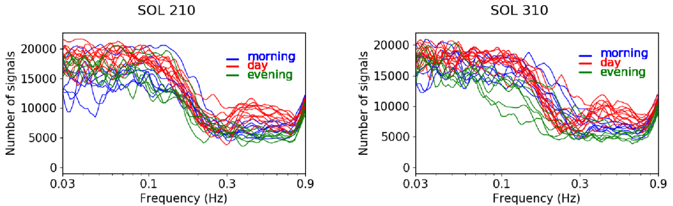
Figure 9. Number of polarized signals detected per hour as a function of frequency in the morning (0:00–7:00, blue curves), during the day (7:00–18:00, red curves), and the evening (18:00–24:00, green curves) on sol 210 (left) and 310 (right).
