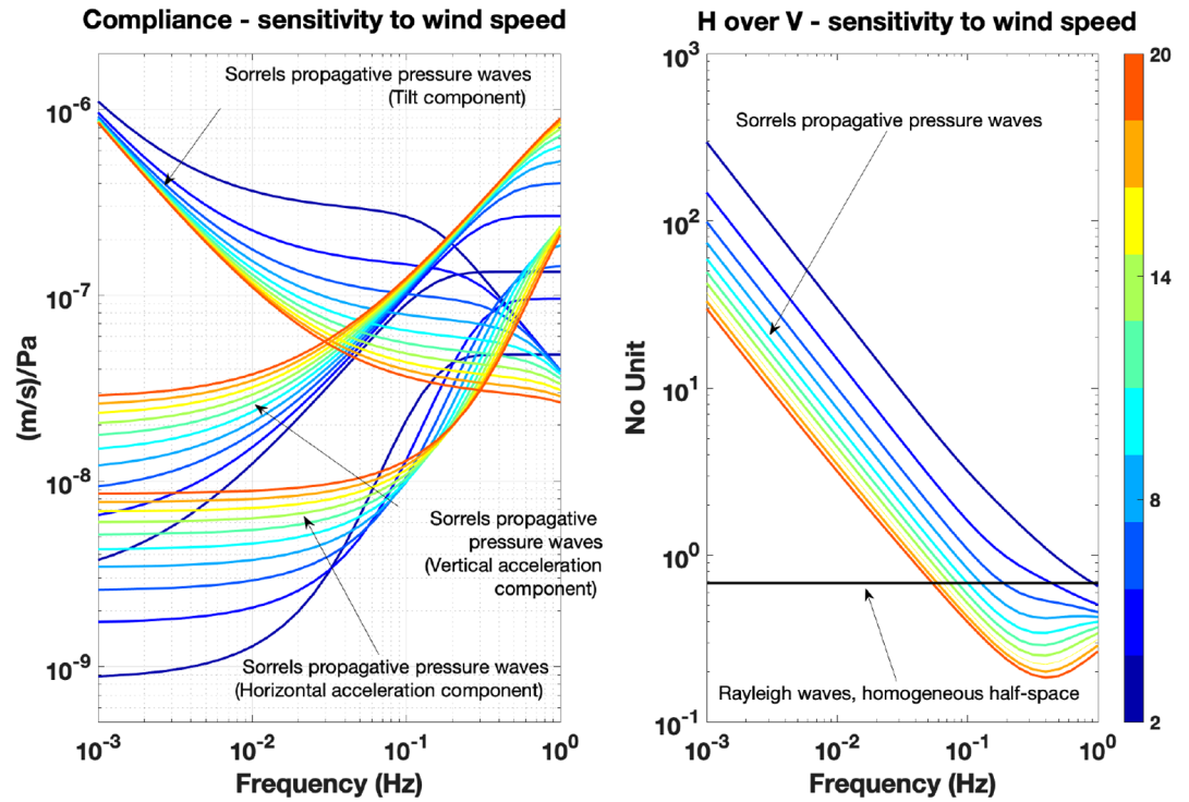
Figure 14. Vertical and horizontal compliances for the two layer model of Kenda et al. (2020). The first layer is 5 m thick with V_p and V_s of 198 and 118 m/s, while the second layer is a semi-infinite layer with V_p and V_s of 926 and 512 m/s, respectively. This model averages the more complex model proposed by Lognonne et al. (2020). The horizontal acceleration is the sum of both the horizontal tilt and of the horizontal ground acceleration and converted to ground velocity. Together with the vertical ground velocity, they are shown for different wind velocities as a function of frequency on the left figure. The color bar represents the range of wind values from 2 to 20 m/s. The right figure shows the amplitude of the H/V ratio. The phase of the H/V for a layered model is the same as for a homogeneous model and equal to -i .
