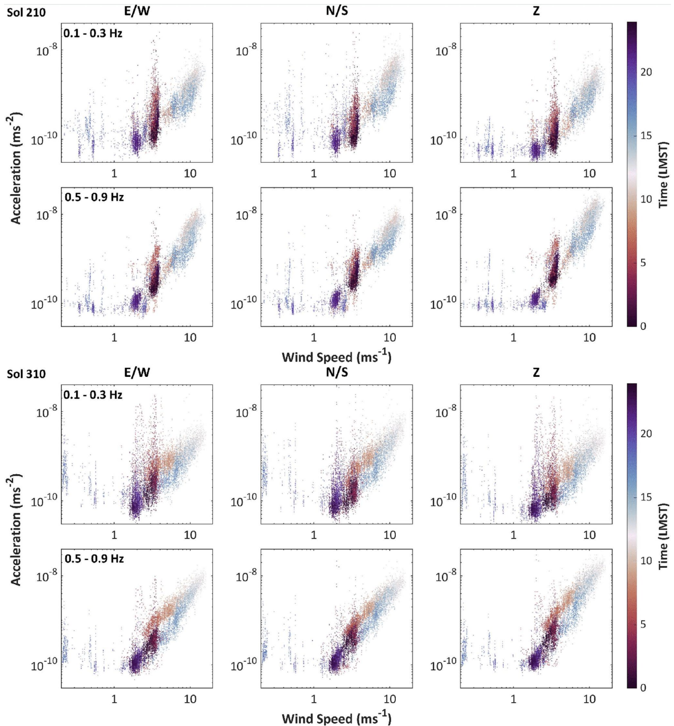
Figure 11. Seismic amplitude rms in acceleration as a function of local wind speed and LMST for each component E/W, N/S, and vertical in the frequency band 0.1–0.3 Hz and 0.5–0.9 Hz Sol 210 is shown on the top and sol 310 on the bottom. Colors correspond to the LMST hours.
