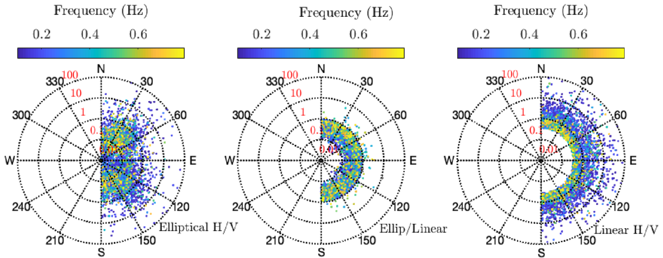
Figure 12. Decomposition of the elliptically polarized signals from sol 210 into elliptical and linear components assuming a phase delay of 0.15 radians between both components. From left to right are shown the H/V ratio of the elliptical components, the ratio between elliptical and linear component and the H/V ratio of the linear component. Shown are only polarized signals with degree of polarization larger than 0.75, frequencies between 0.3 and 0.8 Hz and linearity between 0.85 and 0.95 (B/A ratio between 0.05 and 0.15). This corresponds to signals with small but stable ellipticity. For the selected phase shift, a significant amount of elliptical components is found along the 30°–40° North azimuth and its perpendicular direction. Both, the elliptical and linear component have more signals with H/V ratio below one than above. Most of the signals have more energy on the linear component than on the elliptical component, tending toward equivalent energy at 0.8 Hz.
