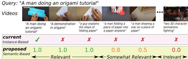
Figure 1: All current video retrieval works treat caption collected for a certain video as relevant, even when other videos are equally relevant to a query text. This makes the evaluation of popular datasets ad hoc at times. We propose to use continuous similarity, allowing multiple videos to be treated as equally relevant. Ex. from MSR-VTT [64].
