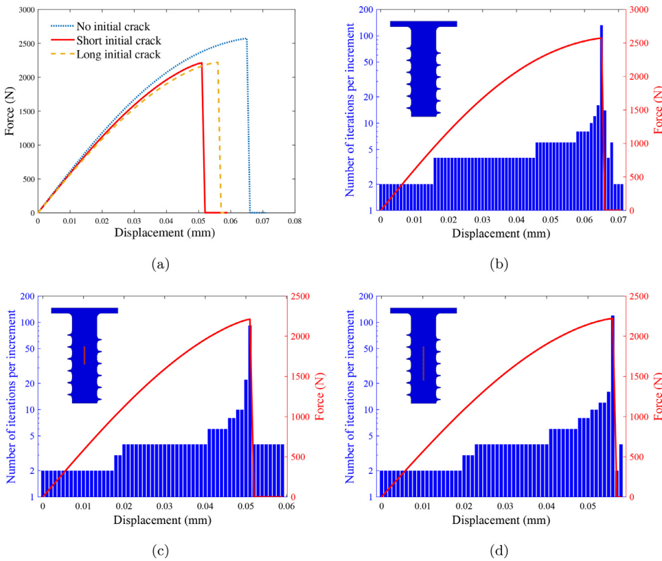
Fig. 9. Screw tension tests: (a) force versus displacement curve for each of the three cases considered, together with the number of iterations per increment for (b) a screw with no initial crack, (c) a screw with a short ( a = 3 mm) initial crack, and (d) a screw with a long ( a = 6 mm) initial crack.
