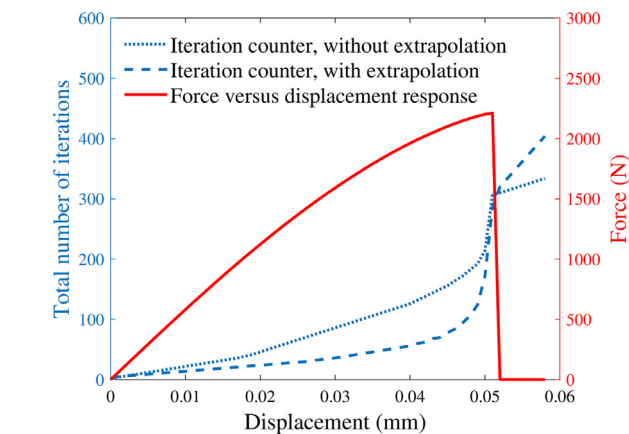
Fig. 10. Screw tension test: assessing the influence of the extrapolation technique. Force versus displacement response and cumulative number of iterations required to achieve convergence with and without extrapolation.
