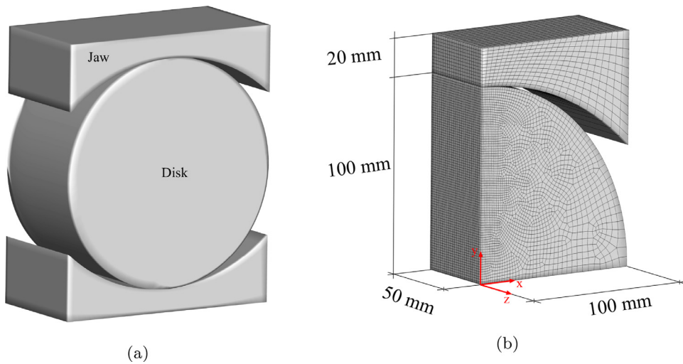
Fig. 11. 3D Brazilian test: (a) complete geometry of the test and (b) geometry, boundary conditions and mesh of the computational model. One-eighth of the problem is simulated, taking advantage of symmetry.
