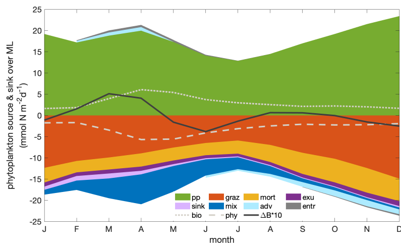
Figure C2. Seasonal cycles of phytoplankton source and sink processes integrated over the mixed layer, along with the net biological fluxes (dotted line) and the net physical fluxes (dashed line), and the tendency (change) of phytoplankton biomass (solid line) integrated over the mixed layer.
