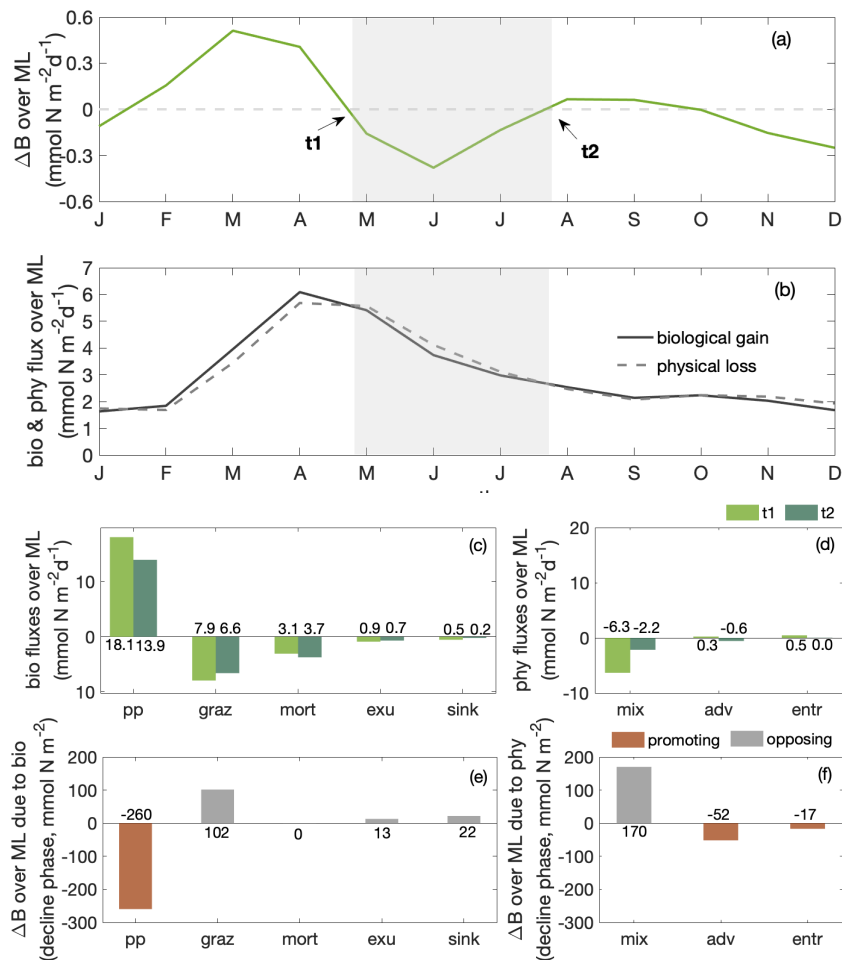
Figure 4. Seasonal cycles of (a) total phytoplankton biomass change \Delta B in the mixed layer (in \text{mmol N m}^{-2} \text{d}^{-1} ); gray shading indicates the decline phase as in Fig. 3, with t_1 and t_2 marking the beginning and end of the decline phase; (b) MLD-integrated phytoplankton net biological and physical fluxes (in \text{mmol N m}^{-2} \text{d}^{-1} , as shown in Eq. 1 plus the entrainment introduced by the integration); bar plots of (c) biological and (d) physical fluxes at the start ( t_1 , light green) and end ( t_2 , dark green) of decline phase; bar plots of the integrated change over the decline phase over mixed layer due to (e) biology and (f) physics within the focus region. Red and grey indicate promoting and opposing ML-integrated phytoplankton biomass decline. pp stands for primary production; graz for consumptive mortality; mort for natural mortality; exu for exudation; sink for sinking; mix for mixing; adv for advection and entr for entrainment.
