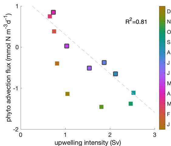
Figure C4. Correlation between upwelling intensity and phytoplankton convergence of advection over the mixed layer. A negative convergence equals a divergence of phytoplankton biomass due to the combined effect of upwelling and lateral transports. Color indicates the time of the year and black edges the decline phase. The correlation coefficient ( R^2=0.81 ) is shown for the decline phase.
