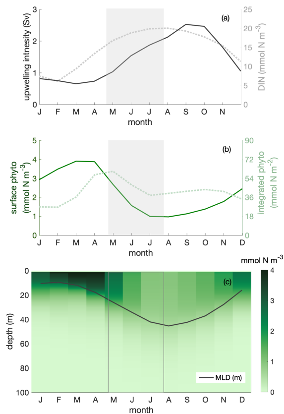
Figure 3. Seasonal cycles of (a) upwelling intensity (in Sv, solid line) and surface dissolved inorganic nitrogen (DIN) concentration (in mmol N m -3 , dotted line); (b) surface (in mmol N m -3 , solid line) and mixed layer depth (MLD)-integrated phytoplankton biomass (in mmol N m -2 , dotted line); (c) phytoplankton depth-month distribution with the seasonal cycle of MLD (in m, solid line) within the focus region. The shaded area indicates the decline phase of MLD integrated phytoplankton biomass.
