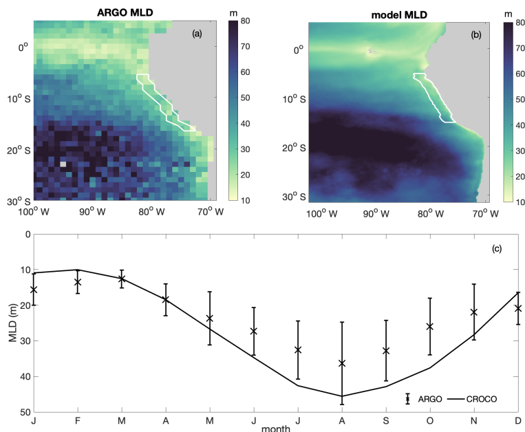
Figure B3. Annual average spatial distribution of mixed layer depth (MLD) from (a) ARGO and (b) CROCO-BioEBUS; (c) Seasonal variation of average mixed layer depth from ARGO (crosses, with lines indicating the standard deviation) and model simulation (line) within focus region. White lines highlight the focus region.
