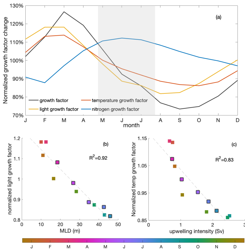
Figure 5. (a) Seasonal cycles of the normalized total (black) growth factor, light (yellow)-, temperature (red)- and nitrogen (blue)-related growth factors, as experienced by phytoplankton over the mixed layer. The grey shading indicates the decline phase; (b) seasonal correlation of MLD and mixed layer averaged light-related growth factor; (c) correlation of upwelling intensity and mixed layer averaged temperature-related growth factor. Colors indicate the time of the year (months) with black edges marking the months of the decline phase. R^2 value of the correlation is shown in the right of the panels
