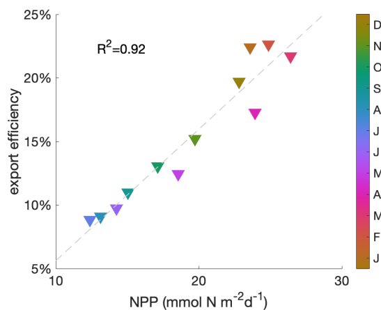
Figure C5. Correlation of export efficiency (defined as ratio of primary production over export below the euphotic layer) with net primary production (NPP). Colors indicate the time of the year.
