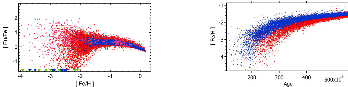
Fig. 2. Left panel: Locations of BHNSMs (green dots/triangles) and NSMs (blue dots/triangles) in the [\text{Eu}/\text{Fe}] vs. [\text{Fe}/\text{H}] plane, whereas red dots represent all model stars. Figure taken from [9]. Right panel: Illustration of a shifted age-metallicity relation. Red (blue) squares represent model stars in a model that does (not) permit failed SNe. A model that permits failed SNe produces less Fe during a given time step, so the [\text{Fe}/\text{H}] enrichment is slowed down as opposed to a model which does not allow failed SNe.
