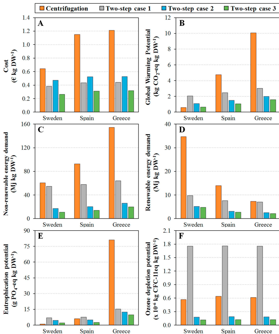
Fig. 3. Impact of C. zofigiensi harvesting process configuration on A. cost, B. global warming potential, C. non-renewable energy demand, D. renewable energy demand, E. eutrophication potential, and F. ozone depletion potential. Baseline case assumes the use of centrifugation only, while two different two-step processes were assessed: Case 1 utilised NaOH, MgSO 4 and HCl, while Case 2 utilised Mg(OH) 2 , Ca(OH) 2 and H 3 PO 4 . Case 3 uses the case 2 chemicals but includes nutrient recycling. All analyses were based on bench scale data from Sections 3.1 and 3.4.
