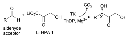
Scheme 1 TK reaction with lithium β-hydroxypropyruvate (Li-HPA 1 ), highlighting the WT-TK S -stereochemistry in the α,α'-dihydroxyketone product.
