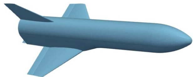
Figure 13: Potential aerodynamic shape for second generation hypersonic flight demonstrator on top of THEMIS
