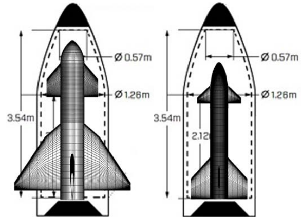
Figure 12: LauncherOne fairing with generic ReFEx successor (left) and current ReFEx geometry (right)
