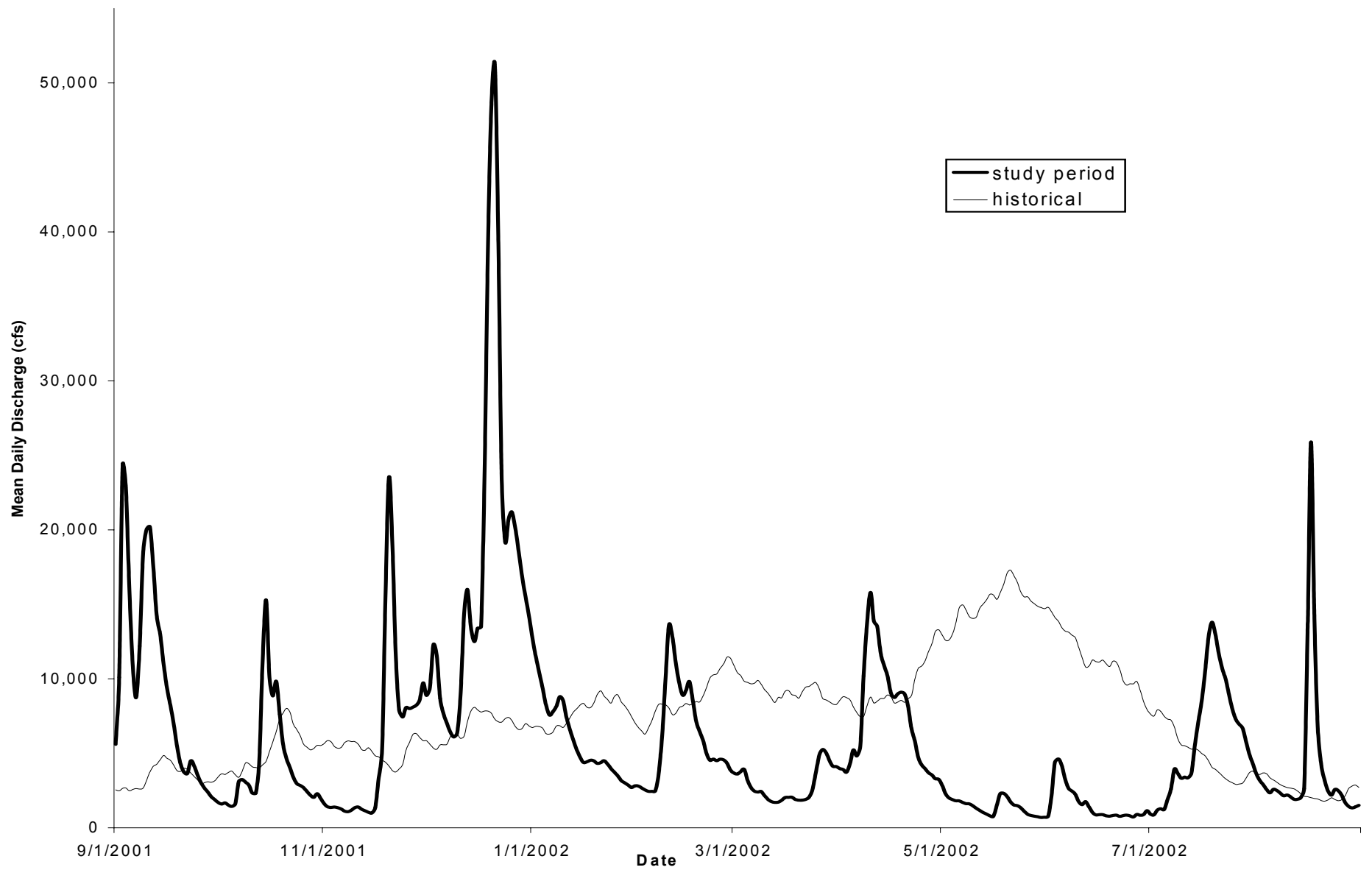
Figure 2. Historical (based on 82 years of record) and mean daily discharge recorded during the study period (September 01, 2001 – August 31, 2002) at the USGS Brazos River at Richmond, Texas gage (station #08114000).
