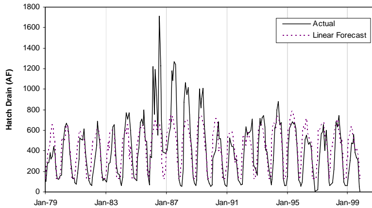
Figure 33. Forecast from Linear Regression for Hatch Drain
