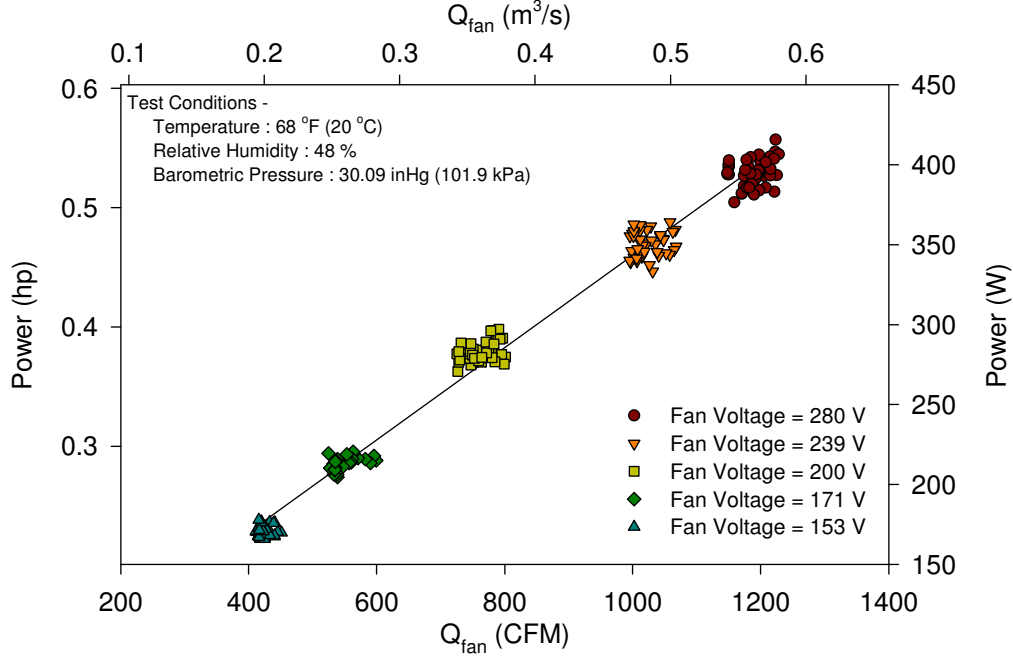
Figure A-24: Fan Power for Series Terminal Unit S8C
