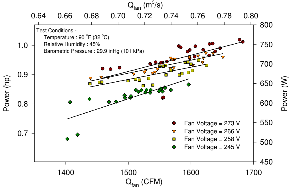
Figure A-23: Fan Power for Series Terminal Unit S12B
