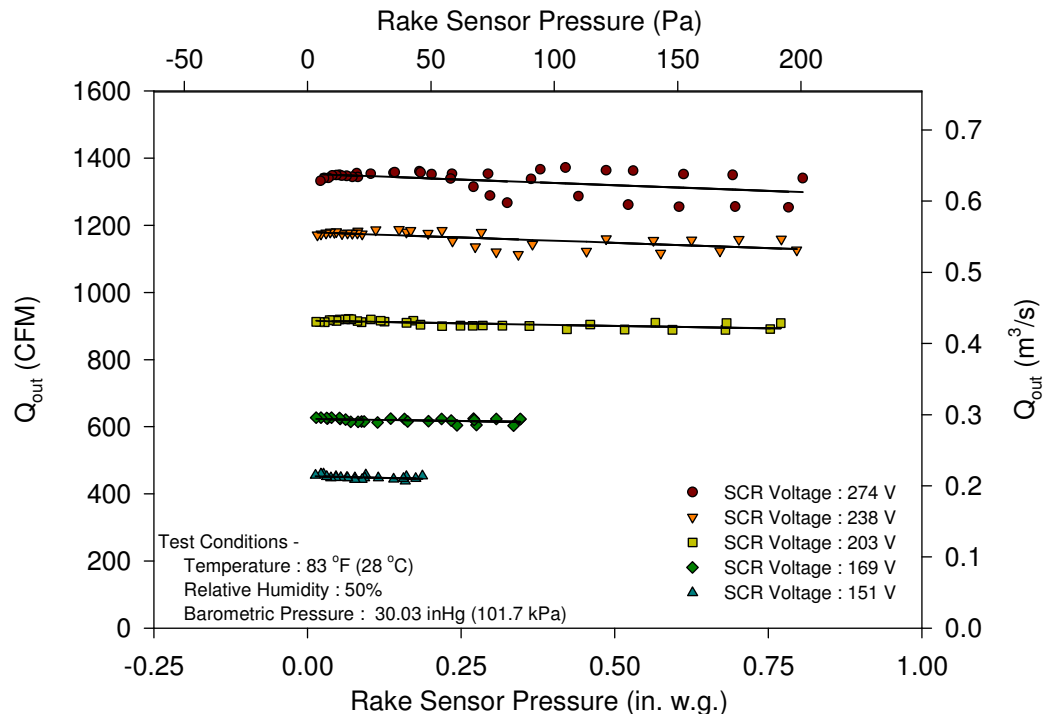
Figure A-16: Fan Airflow for Series Terminal Unit S8B
