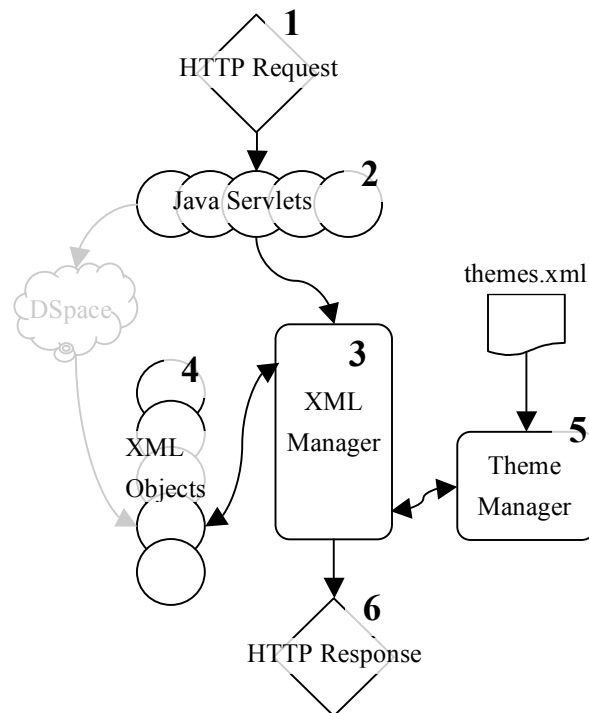
Figure 1: Six stages of an HTTP request
