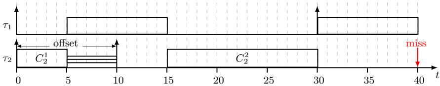
Fig. 8 A schedule to release the two tasks in Table 12 simultaneously. Task \tau_2 in this schedule has longer worst response time than the incorrect schedulability analysis used in Kim et al. (2013), Ding et al. (2009)
