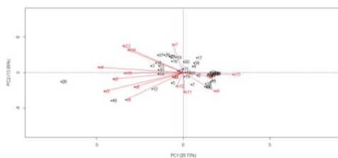
Figure 3. Biplot Analysis graph of America
