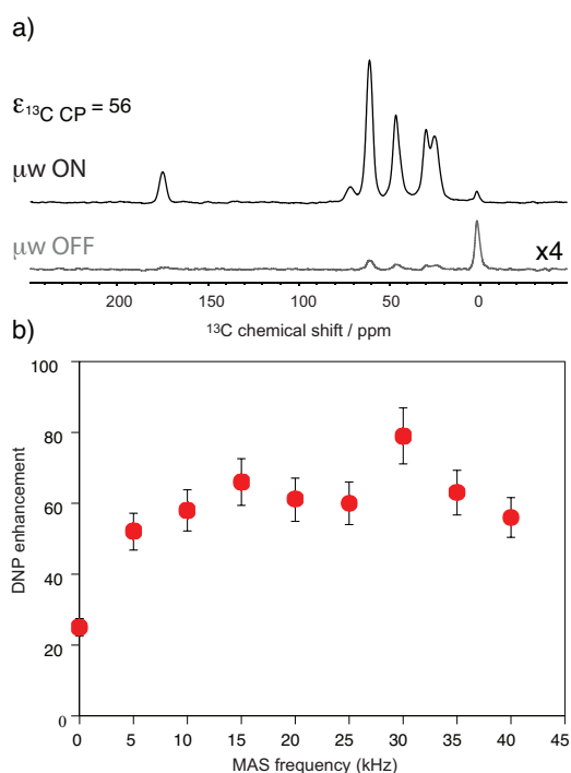
Figure 1: a) ^{13}\text{C} CPMAS NMR spectra of uniformly ^{13}\text{C} -labeled proline (0.25 M proline in glycerol- d_6 /D _2 O/H _2 O, 60:30:10 volume ratio containing 10 mM AMUpol) at 18.8 T and 40 kHz magic angle spinning. The spectra were recorded with (upper spectrum) or without (lower spectrum) \mu\text{w} irradiation at 527 GHz to induce DNP. The resonance at 0 ppm corresponds to the silicon plug insert present at the top of the rotor. For all experiments, the main magnetic field was swept so that the fixed frequency of the gyrotron yielded the maximum enhancement for AMUpol. b) MAS frequency dependence of the DNP enhancements measured from ^{13}\text{C} CPMAS experiments measured on the proline resonances. A small amount of solid KBr was added (see details in the SI) to the rotor to monitor sample temperature by measuring the ^{79}\text{Br} T_1 relaxation time. [20] A sample temperature of 115 \text{ K} \pm 3 was maintained over the whole spinning range for both microwave ( \mu\text{w} ) on and off experiments. The reported enhancements correspond to the mean value of the enhancement factors measured on the 5 carbon-13 resonances of proline. All measurements were performed with 16 W of microwave power at the probe.
