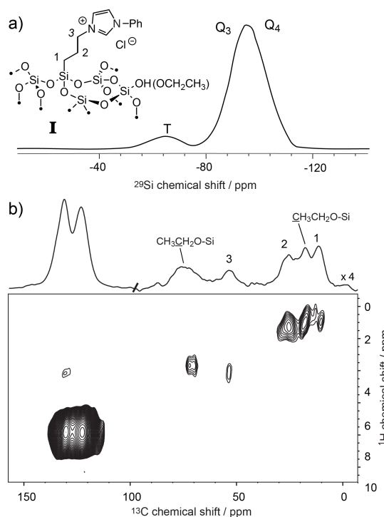
Figure 3: a) One-dimensional 29 Si DNP-SENS CP-CPMG spectrum of I , recorded at 18.8 T (800 MHz) and 40 kHz MAS. The sample was impregnated with a solution of 10 mM AMUpol in 90:10 D 2 O/H 2 O, T \approx 115 K. During acquisition, SPINAL-64 decoupling [21] was applied with a rf amplitude of 130 kHz. The cross-polarization (CP) contact time was 3 ms and the number of scans was 256 (total acquisition time 17 minutes). The CP-CPMG spectrum is shown in its echo reconstructed form and was obtained by summing the whole echoes of the FIDs in the time domain, followed by Fourier transform and application of a first-order phase correction. A total of 40 echoes were acquired. b) Contour plot of a two-dimensional 1 H- 13 C spectrum of I recorded with DNP at 18.8 T (800 MHz) and 40 kHz MAS. A total of 38 t_1 increments of 40 \mu s with 256 scans each were recorded. The CP contact time was 700 \mu s, and the polarization-buildup interval was 4 s. The total experimental time was 10.8 hours. SPINAL-64 heteronuclear decoupling was applied during t_2 with an rf amplitude of 100 kHz. During t_1 , eDUMBO-1 22 [22] homonuclear decoupling was applied with an rf amplitude of 150 kHz. A scaling factor of 0.56 was applied to correct the 1 H chemical shift scale.
