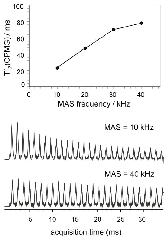
Figure 4: Plot of T_{2\text{CPMG}} of Q_{3/4}(^{29}\text{Si}) sites as a function of the spinning frequency together with the free induction decays (FIDs) of ^1\text{H}-^{29}\text{Si} CP/CPMG experiments recorded at 10 and 40 kHz MAS frequency. SPNAL-64 decoupling at 130 kHz RF field was applied during acquisition. The other experimental details were the same as those given in the caption of Fig. 3a.
