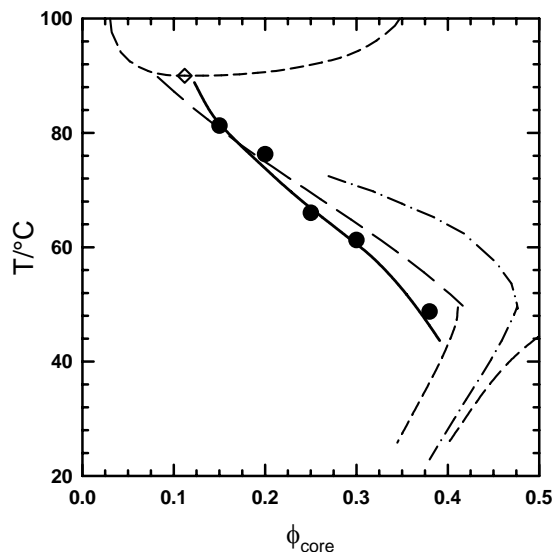
Figure 5.1. Phase diagram showing gas-liquid and liquid-solid coexistence (--) and critical point ( \diamond ); percolation thresholds from MC simulations (— \bullet ), 85 theory (—), 86 and transitions in short time self diffusivity ( \bullet ); glass lines (— \cdot\cdot ). 77
