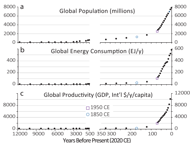
Fig. 1 Correlation of global human population, energy consumption and productivity during the Holocene and Anthropocene epochs. a Global human population (millions), b global energy consumption (EJ/y), and c global productivity ( \$/\text{y}/\text{capita} ), across the Holocene and proposed Anthropocene epochs (in this paper starting in 1950 CE). All three parameters are highly correlated (Spearman's rank coefficient = 1.00). Larger circle = 1850 CE; large square = 1950 CE. Data references are listed in Supplementary Online Material.
