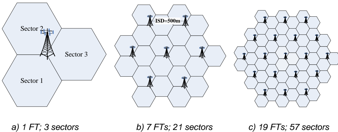
Figure 7. Hexagonal grid network layouts for different FT configurations. Each FT coordinates three sectors.
