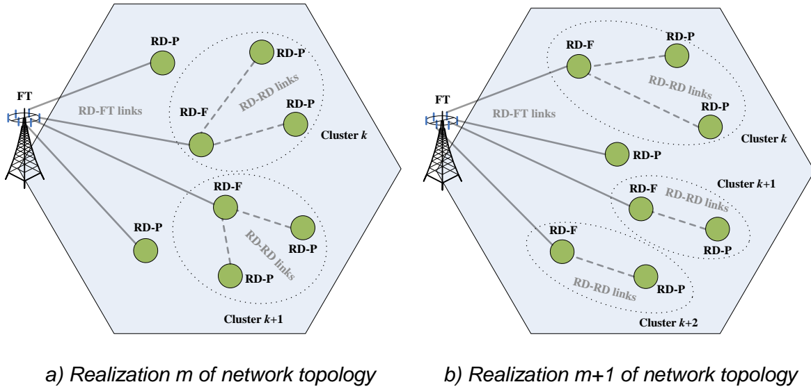
Figure 6. A simplified illustration of different DECT-2020 network node roles and link types within a single FT sector. The role of nodes can vary and is not a fixed node ability. The actual simulated number of RDs within a single FT sector is 72 169 which results in the density of 1 million nodes per \text{km}^2 for \text{ISD} = 500 \text{ m} .
