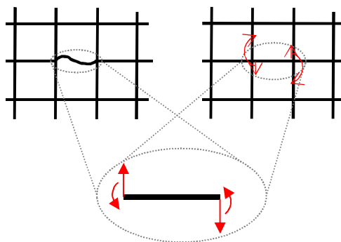
Figure 1 FAM procedure.
