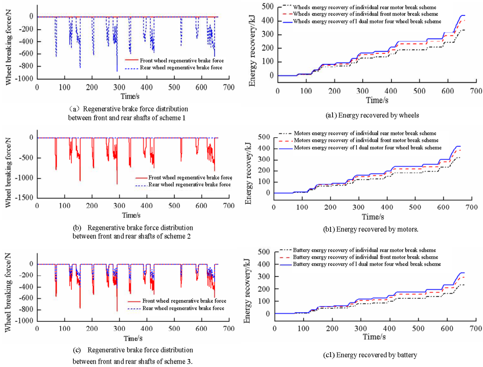
Figure 9 Effect of regenerative brake strategy on regenerative brake force distribution and energy recovery (based on a series parallel brake system).
