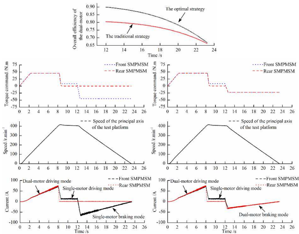
(a) The traditional braking force distribution A (b) The optimal braking force distribution A_1
