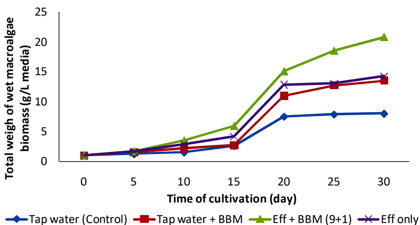
Figure 3 Growth curve of macro-algae Oedogonium sp cultivated in four different culture media: tap water as control, tap water + BBM, effluent produced in this study with the addition of BBM (9:1 v/v), and effluent without BBM.
