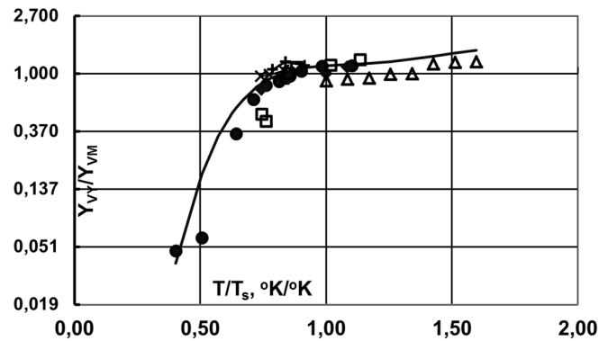
Figure 7 Correlation of Y_{VY}/Y_{VM} at various temperatures T/T_s , data from [11,19,21-24], and the line fitted model Eqs. (19) and (20).
