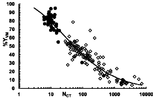
Figure 3 Fitted correlation % mass fraction of released volatile matter \%Y_{VM} in the proximate analysis for new coal type number N_{CT} from Eqs. (10) and (11) for coal and biomass types from the databank.
