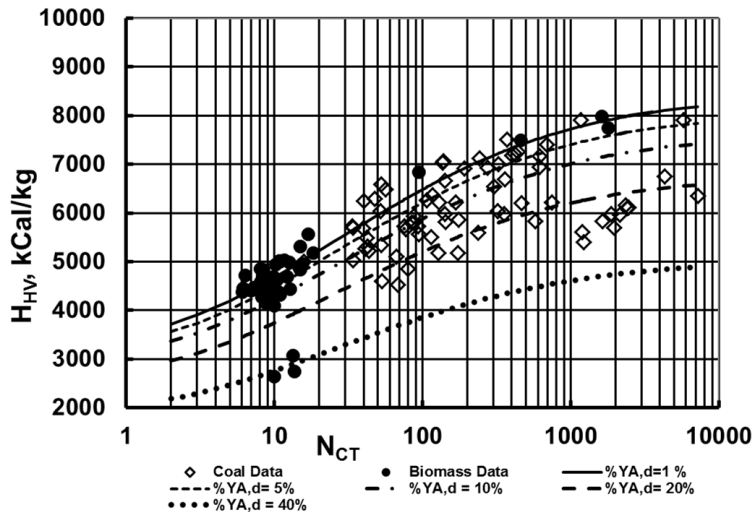
Figure 4 Predicted high heating values of dry coal and biomass correlated to coal type number N_{CT} and ash content \% Y_{A,d} .
