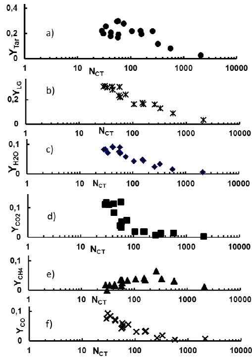
Figure 6 Correlations of light gas Y_{LG} , Y_{tar} , and components Y_{H2O} , Y_{CO2} , Y_{CH4} , and Y_{CO} yield with coal type number N_{CT} . Measured data from Xu and Tomita [6].
