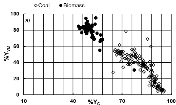
Figure 2 Correlation of the mass fraction of released volatile matter in the proximate analysis with the carbon content of the coals and biomass from the databank.
