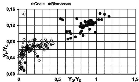
Figure 1 Van Krevelen diagram for coals and biomass in the databank.
