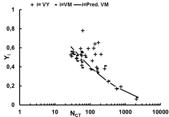
Figure 5 Correlation of volatile yield Y_{VY} and volatile matter mass fraction in proximate analysis Y_{VM} with the coal type number N_{CT} and predicted volatile matter mass fraction (Pred. VM) using Eqs. 10 and 11. Measured data from Xu and Tomita [6].
