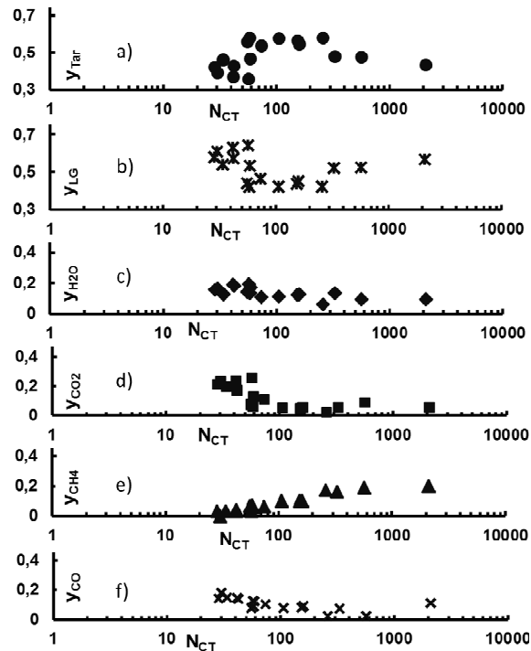
Figure 8 Generated correlations of mass fractions of light gas y_{LG} , tar y_{Tar} , y_{H2O} , y_{CO2} , y_{CH4} and y_{CO} in the total volatile matter yield when compared with N_{CT} . Measured data from Xu and Tomita [6].
