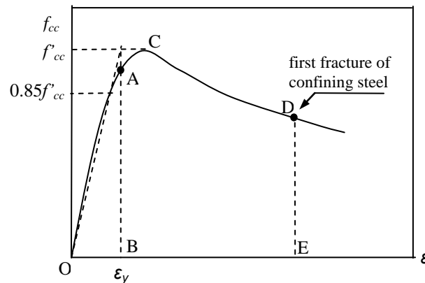
Figure 5 Ductility measurement.
