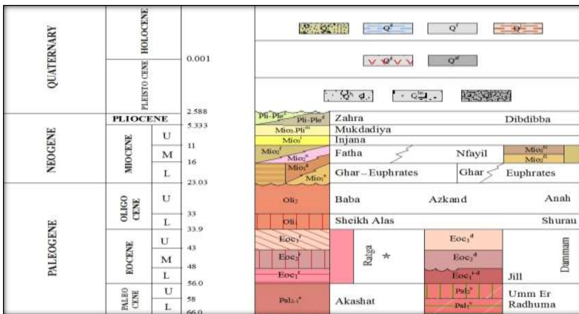
Figure (2): Geological map of the studied area (after Sissakian, V.K et al, 2015): (a) exposed geological formation; (b) stratigraphic column.
