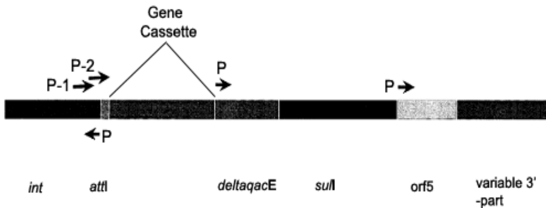
Figure 1. Schematic of a Class 1 integron*.
