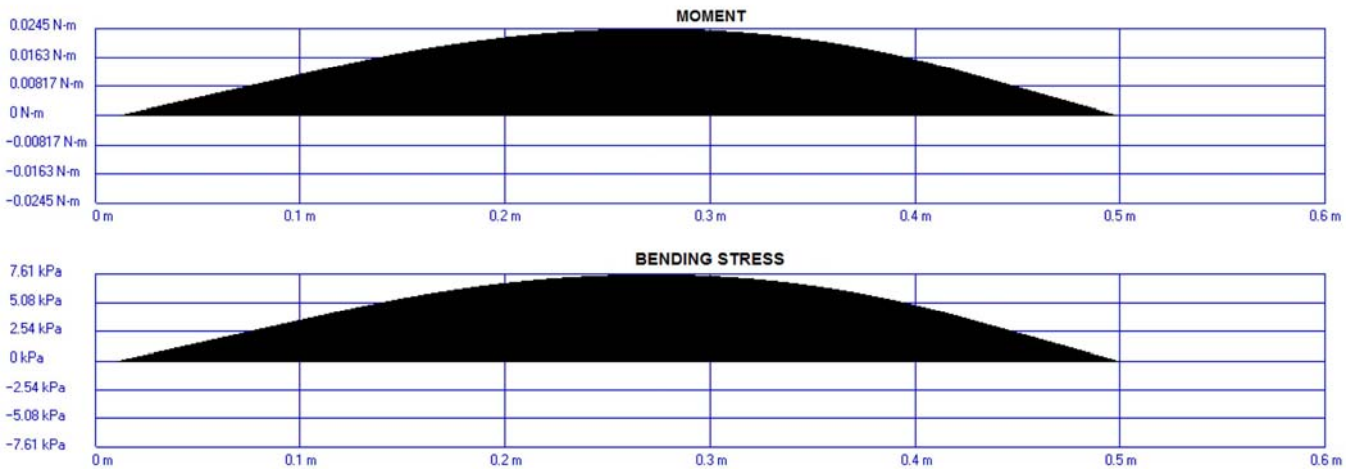
Figure 1b Bending moment and stress diagrams of the screw shaft
