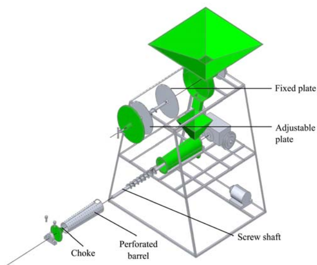
Figure 3 Exploded view of the motorized ginger juice expression machine
