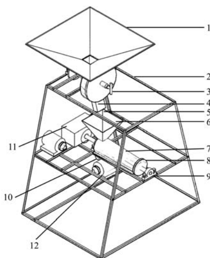
1. Pulverizing hopper 2. Frame 3. Adjustment knob 4. Pulverizing unit 5. Pulverized ginger outlet 6. Expression hopper 7. Expression unit 8. Chaff outlet 9. Bearing 10. Juice outlet 11. Speed reduction gear 12. Electric motor
