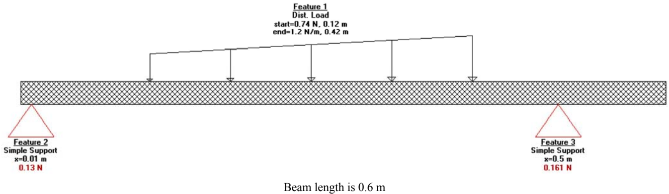
Figure 1a Free body diagram of the screw shaft showing loads and reactions
