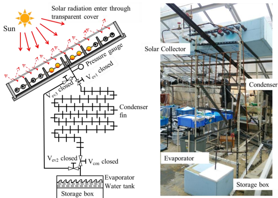
Figure 1 A solar adsorption cooling storage system
