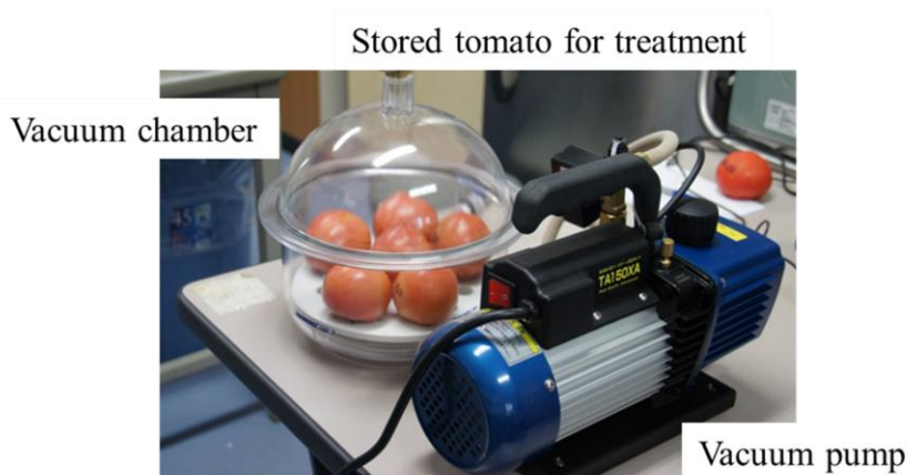
Figure 2 A low pressure treatment process
