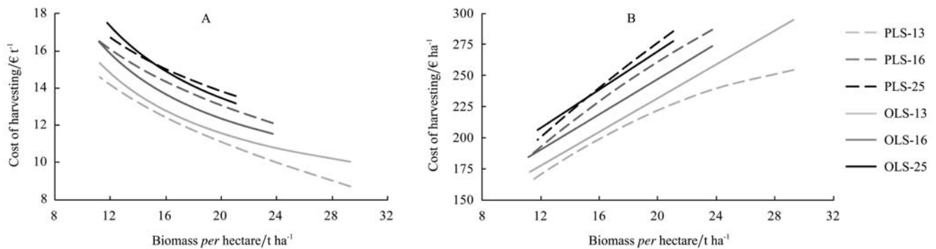
Figure 4 Comparison between OLS and PLS approaches on the cost analysis of the harvesting in relation to production of biomass per hectare of the plantation for three hypothesis of harvesting yard: A - Cost per ton (€ t -1 ); B - Cost per hectare (€ ha -1 )
