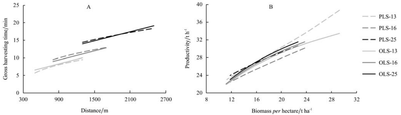
Figure 3A Gross harvesting time predicted by PLS and OLS for three yard sites in relationship with the distance per load .
