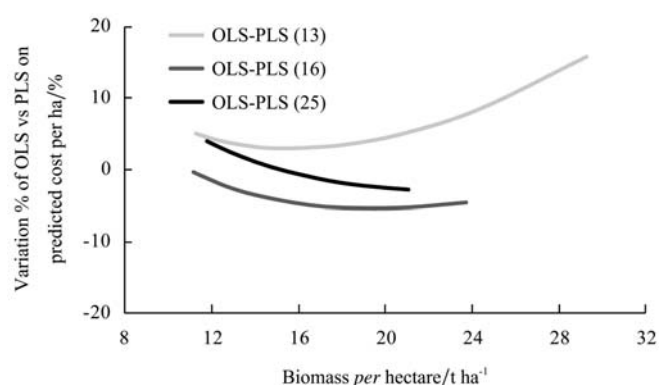
Figure 5 Comparison between OLS and PLS approach on the cost analysis of the harvesting in relation to production of biomass per hectare of the plantation for three hypotheses of harvesting yards
