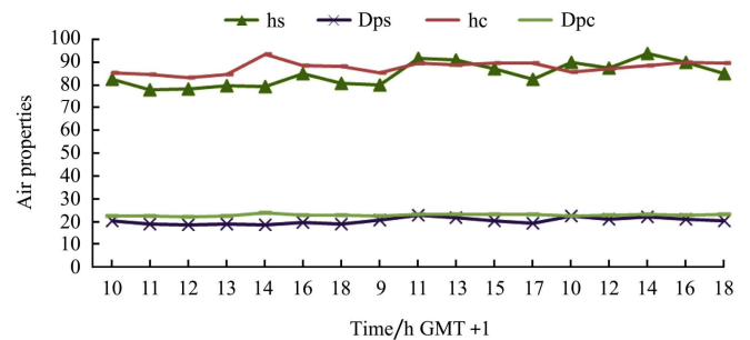
Note: hs is enthalpy of the air entering the pad ( \text{kJ kg}^{-1} ); Dps is dew point temperature of air entering the pad; hc is enthalpy of the air leaving the pad ( \text{kJ kg}^{-1} ); Dpc is dew point temperature of air leaving the pad
