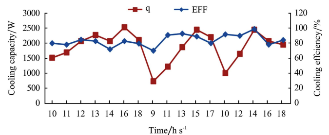
Note: q = cooling capacity (W); EFF = efficiency (%)
