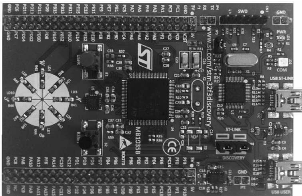
Fig. 3. View of the 32-bit development board of the STM32F303CTV6 ARM Cortex-4M microcontroller
