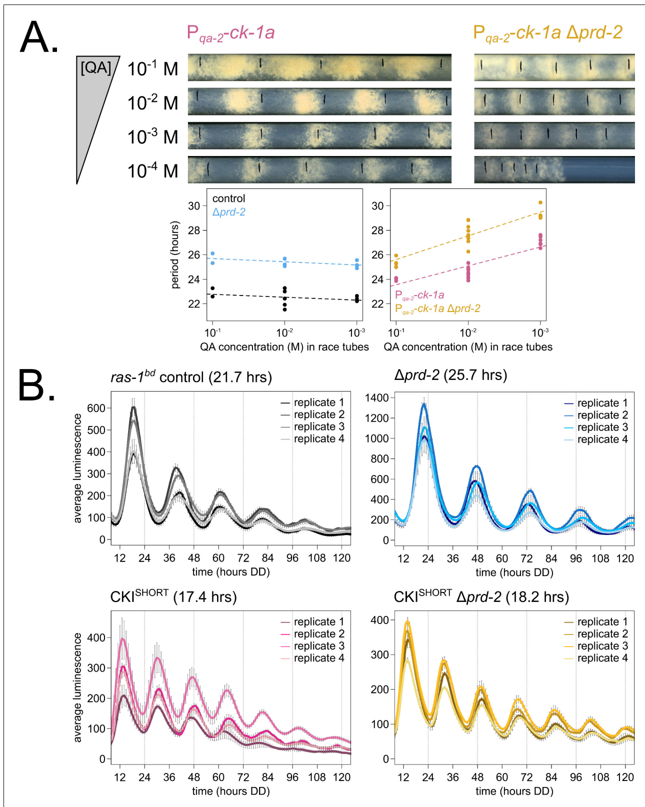
Figure 4. Genetically increasing casein kinase I (CKI) levels or activity rescues the \Delta prd-2 long period phenotype. Representative race tubes (RTs) from ras-1^{bd} P_{qa-2-ck-1a} single (pink) and ras-1^{bd} P_{qa-2-ck-1a} \Delta prd-2 double (yellow) mutants are shown with growth using the indicated concentrations of quinic acid (QA) to drive expression of ck-1a . All results are shown in a scatterplot, where each dot represents one RT's free running period length. ras-1^{bd} controls (black) had an average period of 22.5 \pm 0.5 hr ( N = 12 ), and period length was not significantly affected by QA concentration (ANOVA). Figure 4 continued on next page
