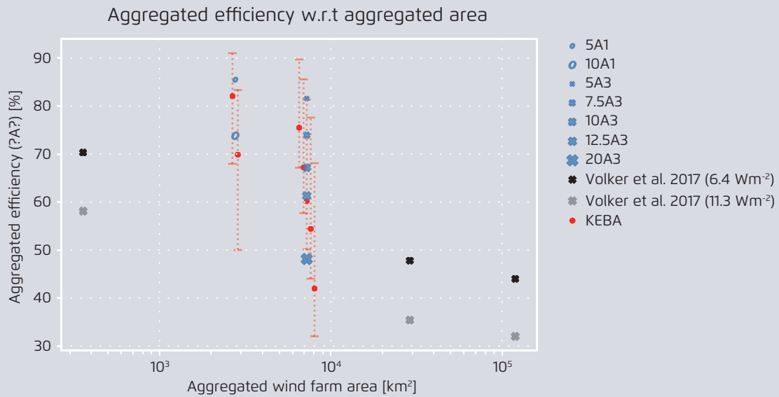
Aggregated relative efficiency relative to total wind farm area in different scenarios
