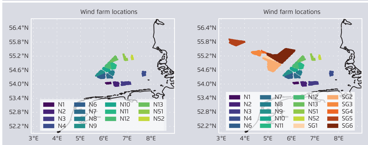
Maps showing the representation of wind farms in inner area A1 (left) and in the inner and outer areas A3 (right).
