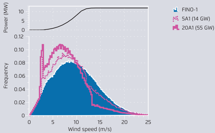
Change in wind speed frequency estimated for different scenarios (bottom) and power curve for the assumed 12 MW turbine (top)
