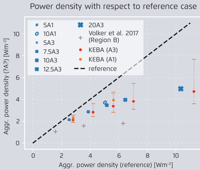
Aggregated generated power density relative to reference power density (no wake) in different scenarios
