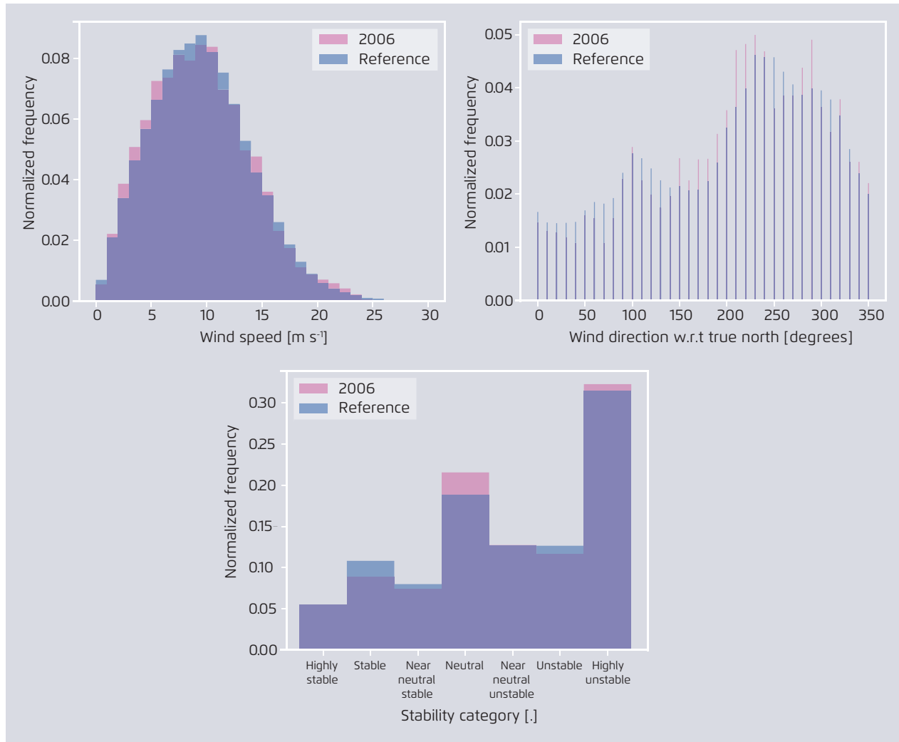
Comparison of distributions of wind speed (top left), wind direction (top right), and boundary layer stability (bottom) for the simulation year (2006) and the reference period
