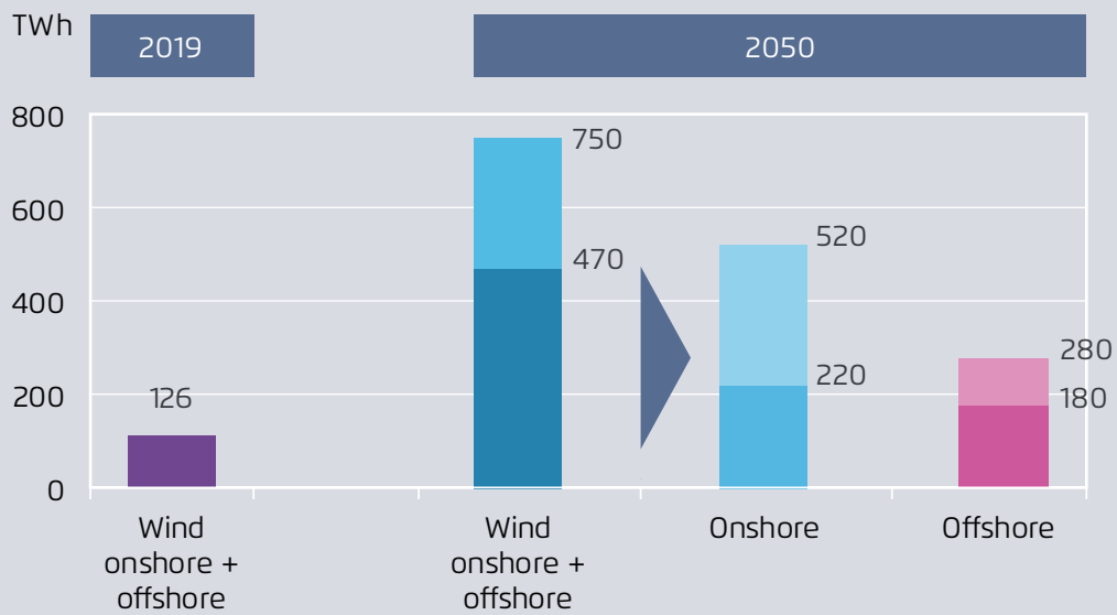
Ranges of necessary wind power generation by 2050 in 95% decarbonization scenarios for Germany in TWh
