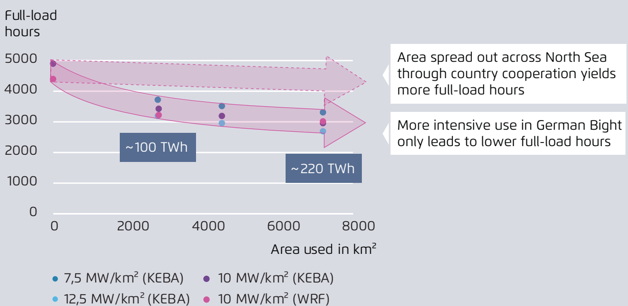
Full-load hours achievable depending on area for offshore wind deployment in the North Sea (and expected yield in TWh)
