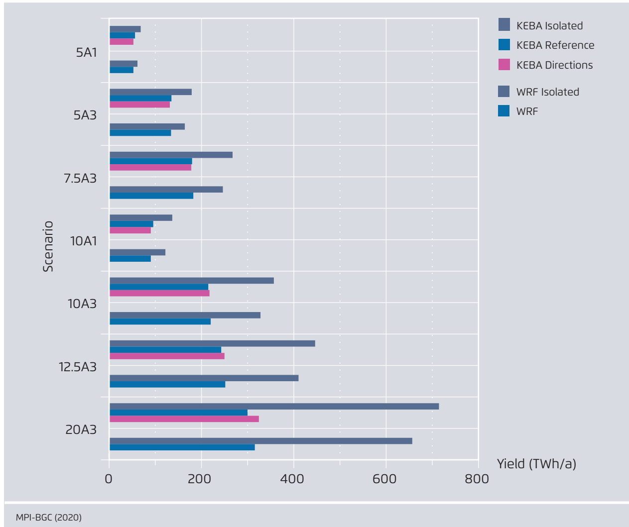
Comparison of yield estimates between the WRF and KEBA methods ("Reference" and "Directions" cases)
