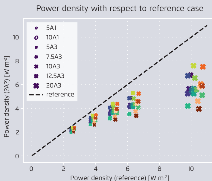
Modelled generated power density compared with nominal reference (no wake) power density in the different scenarios
