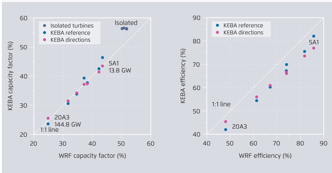
Comparison of WRF estimates with KEBA estimates (“Reference” and “Directions” cases) for capacity factors and efficiencies
