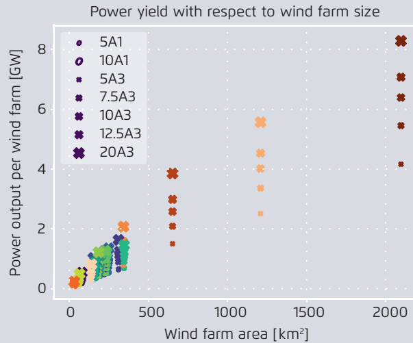
Mean wind farm power output against wind farms area in different scenarios
