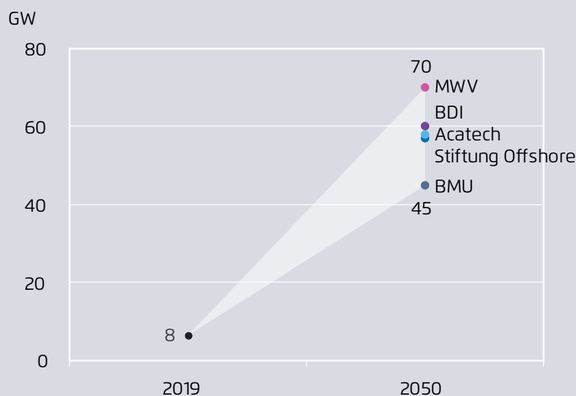
Installed offshore wind capacity for Germany's 95% climate target scenarios in GW
