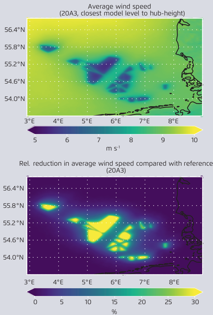
Maps showing the mean velocity (top) and relative difference of wind speed relative to the reference (bottom) at approximately hub height for scenario 20A3 during the entire simulation period for 2006
