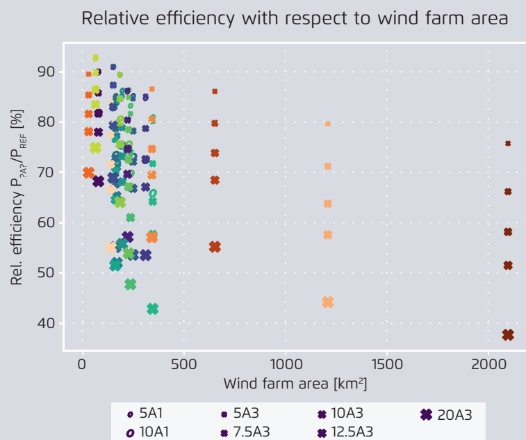
Wind farm efficiency relative to wind farm area in different scenarios
