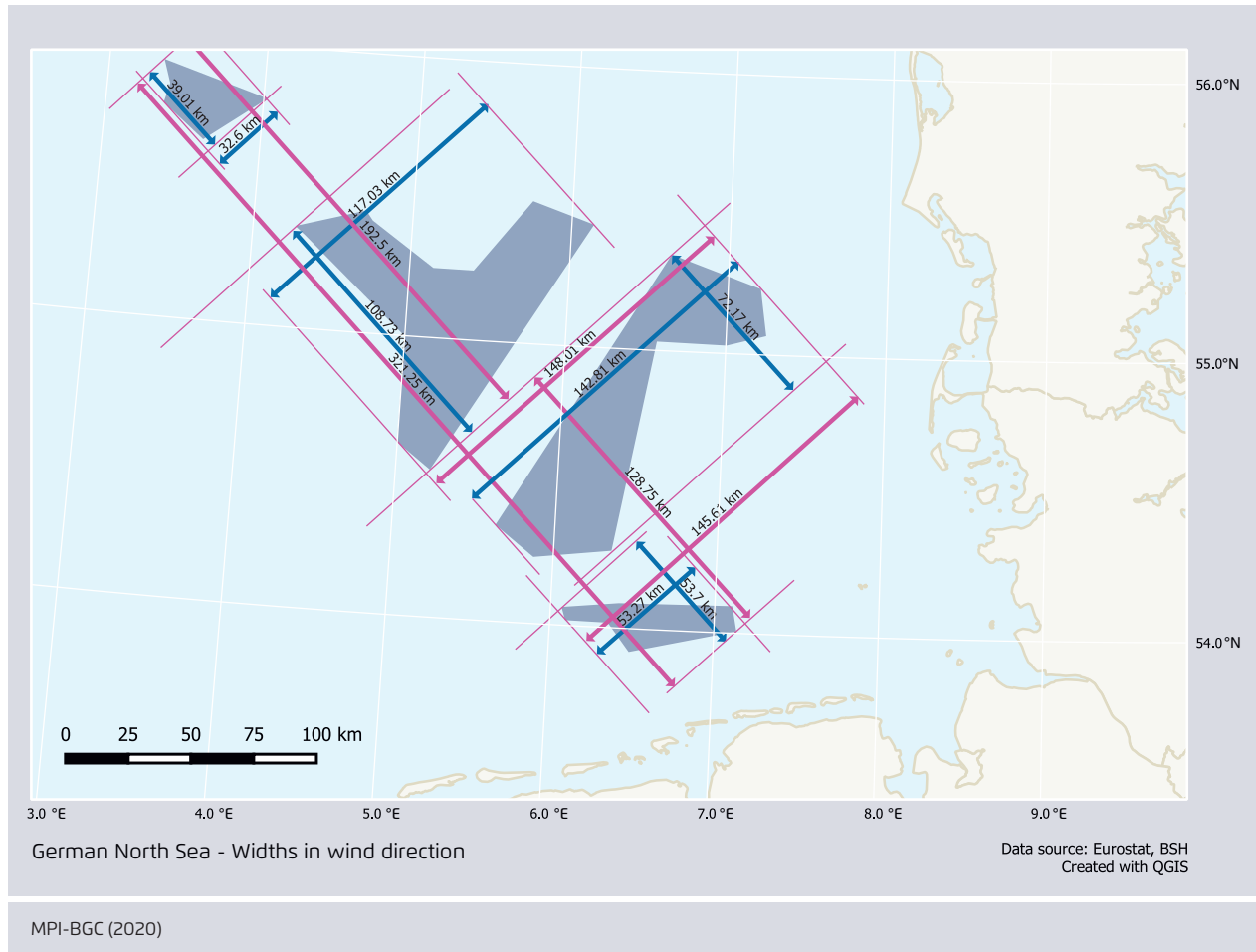
Dimensions of cross-sectional widths and downwind lengths used in the KEBA "directions" estimates for the wind directions NW, NE, SW, and SE
