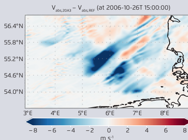
Map showing the difference between wind speed at approximately hub height for scenario 20A3 and the reference simulation for 15:00 GMT on 26 October 2006
