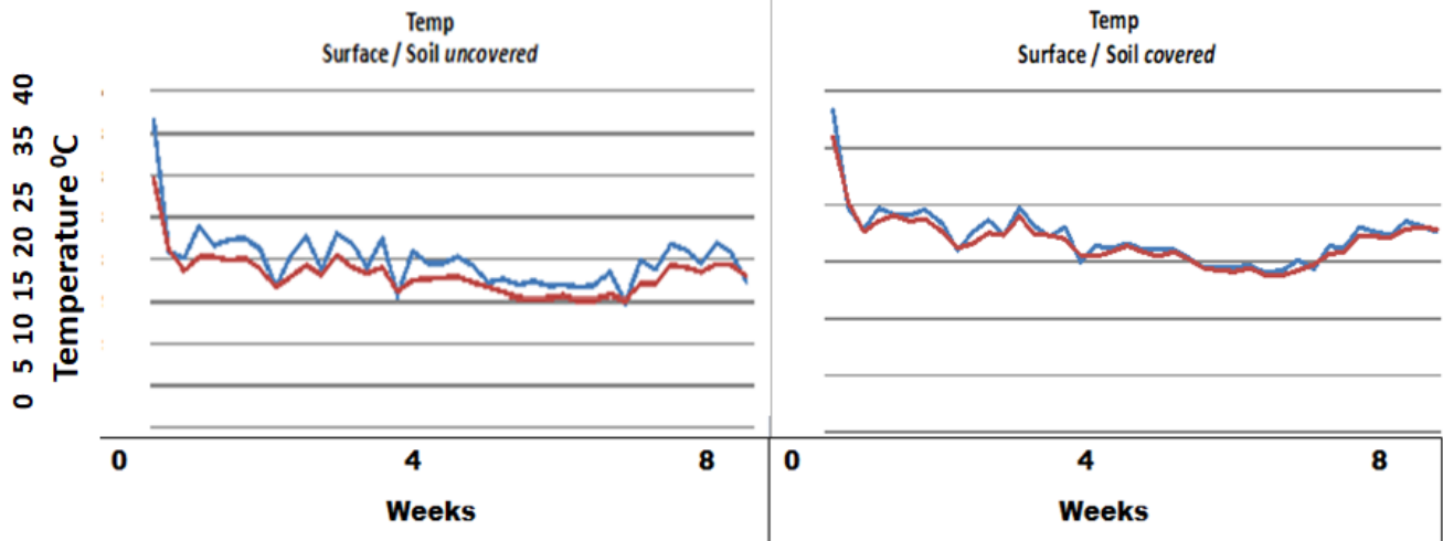
Fig. 1. Temperature gradient recorded over 8 weeks after Mathiola plug transplant into covered and uncovered poly tunnel field soils. Thermal ramp recordings of surface and subsurface (3.0-5.0 cm deep) soils just closest to Mathiola incana plant plug stem base / emerging root zone (MPHRZ) in uncovered or polythene sheets covered regimes in poly tunnel field cultivation system.
