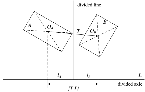
Figure 6. Intersecting test between OBB.
