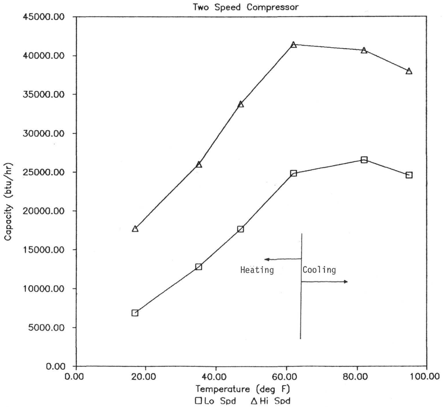
Figure 5.1- Typical capacity performance to a two speed compressor
