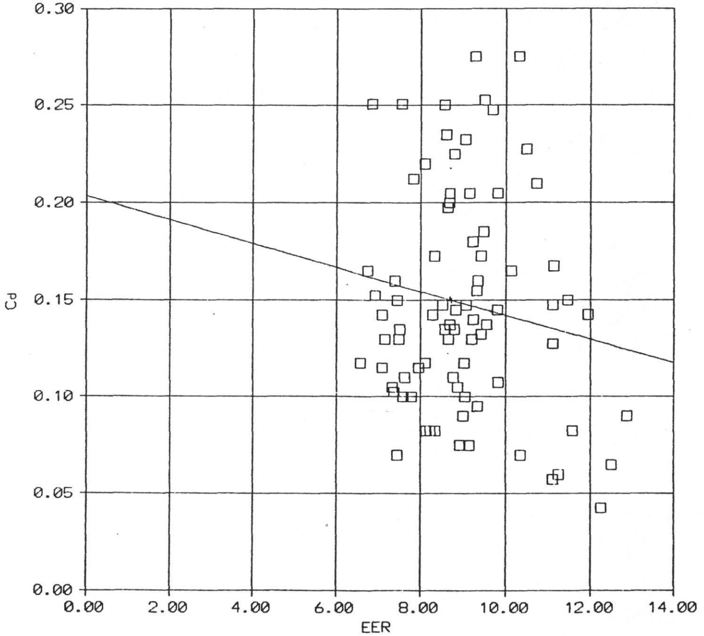
Cd as a function of EER( r^2 = .0238 )
