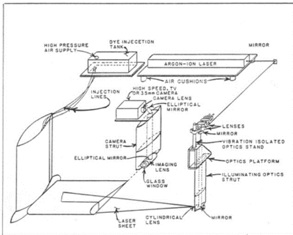
Figure 1 Flow Visualization System
