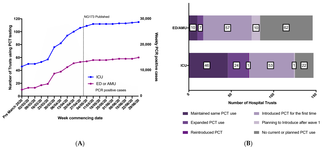
Figure 1. Changed use of PCT testing at acute NHS hospitals in England and Wales. (A) Weekly number of hospitals using procalcitonin (PCT) on intensive care unit (ICU) (---) and Emergency Department (ED)/Acute Medical Unit (AMU) (---). For reference, the time course of the COVID-19 pandemic first wave in England is shown as weekly number of PCR positive cases (---). NG173 = National Institute for Health and Care Excellence (NICE) COVID-19 rapid guideline NG173: [9] Data extracted from Public Health England (PHE) national COVID surveillance reports available at: https://assets.publishing.service.gov.uk/government/uploads/system/uploads/attachment_data/file/916994/COVID19_Weekly_Report_09_September_2020.pdf (accessed on 21 February 2021). (B) Breakdown of changes in PCT use on ICU and ED/AMU at 148 hospitals over the course of the pandemic first wave.
