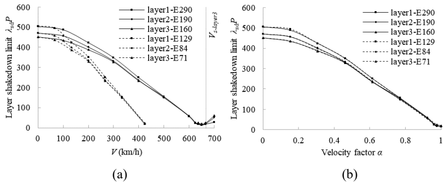
Fig. 4.4 Effect of train speed on dynamic shakedown limit when h_2=2.3\text{m}
