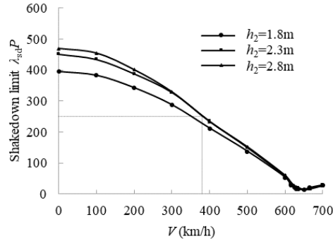
Fig. 4.5 Effect of subgrade thickness on dynamic shakedown limit
