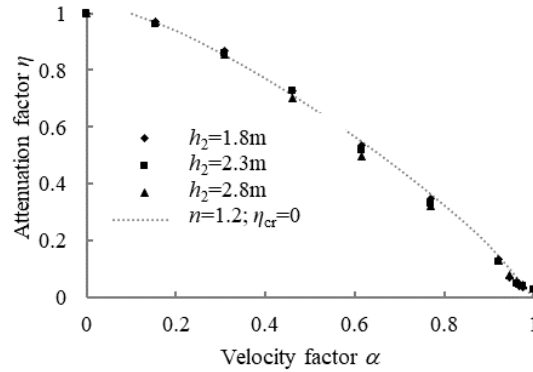
Fig. 4.8 Effect of subgrade thickness on attenuation factor
