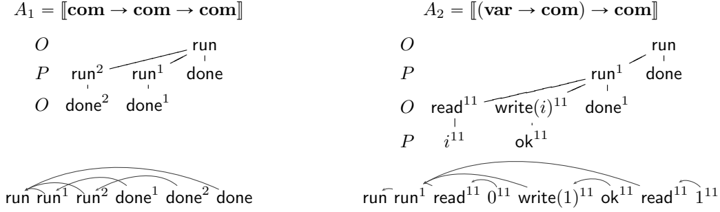
Fig. 4. Arenas and justified sequences
