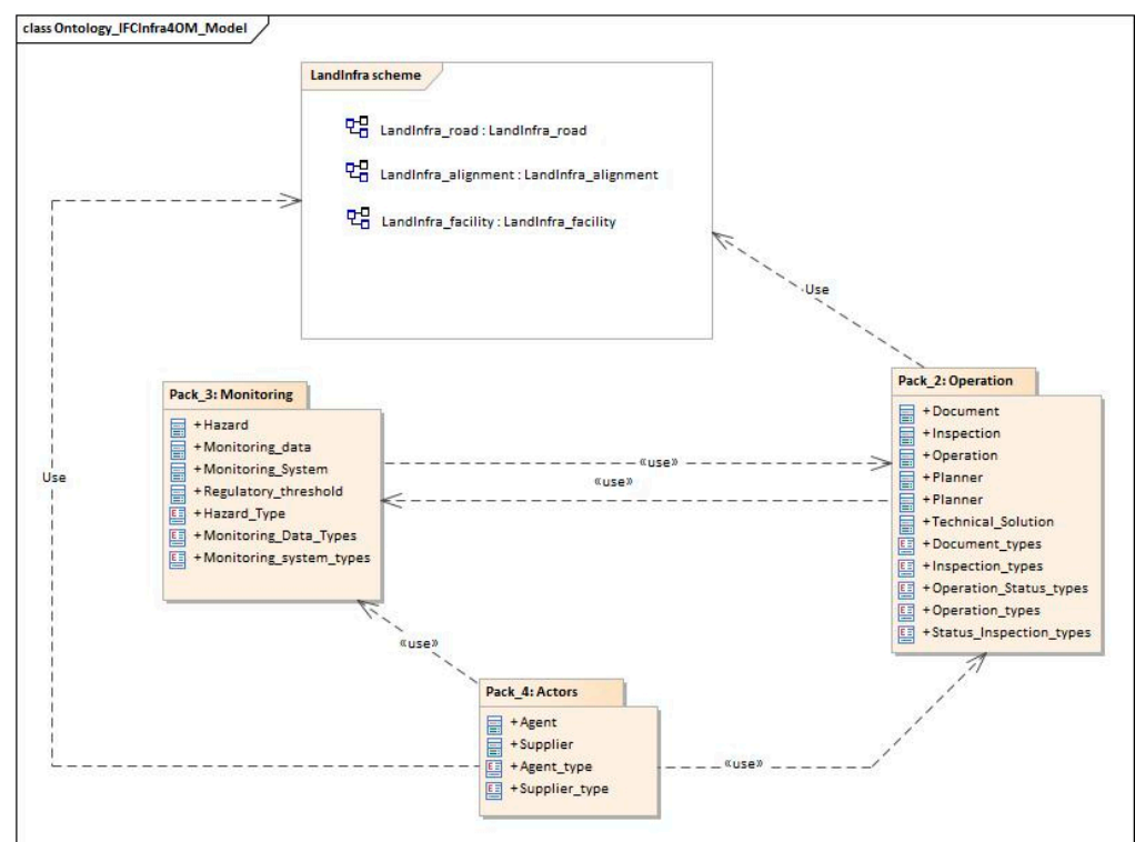
Figure 11. IFCInfra4OM Packages Diagram.
